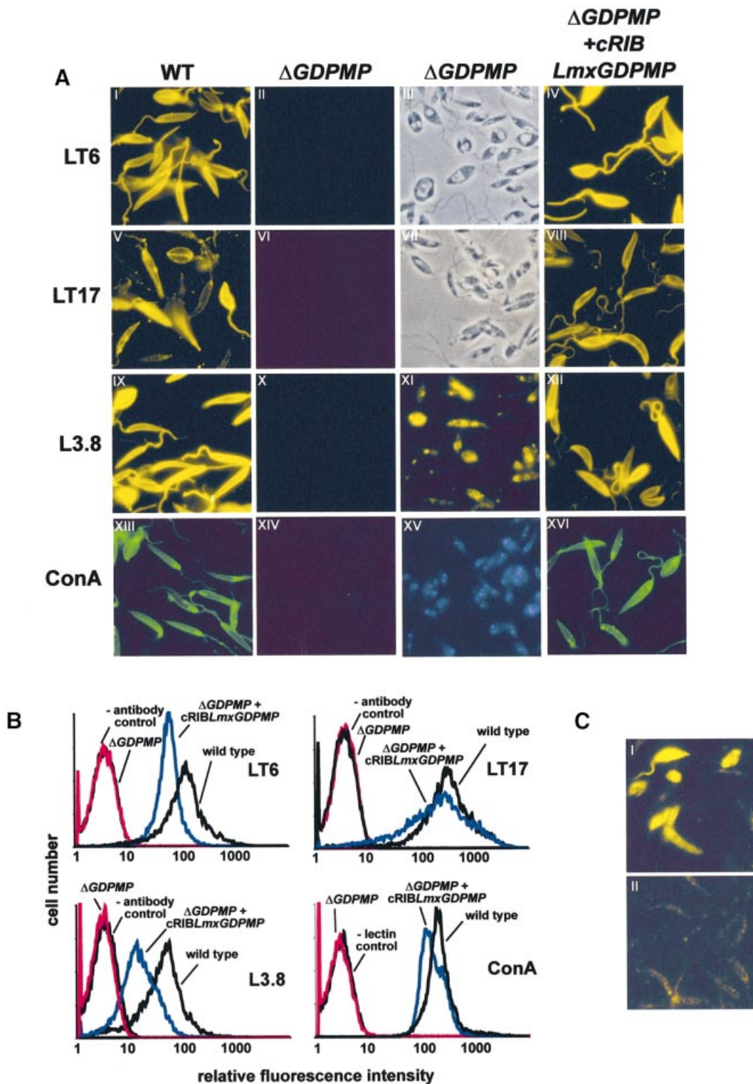
Fig. 5. Immuno-/lectin fluorescence microscopy and FACS analysis of Leishmania WT and mutant promastigotes. (A) Immuno-/lectin fluorescence microscopy of fixed L. mexicana promastigotes. The cells were not permeabilized, except for XI. The parasite lines and the mAbs/lectins used are indicated by the labeling of columns and rows. Exposure times within rows (A) are identical, except for XI, which is \sim 20\times overexposed compared with IX. III and VII in (A) are phase-contrast light microscopy images of II and VI, respectively. (B) FACS analysis of live L. mexicana promastigotes. The parasite lines and the mAbs/lectins used are indicated in each panel. (C) IFM of saponin-permeabilized L. mexicana WT promastigotes labeled with rabbit anti-GDPMP serum (1:200) (I) and pre-immune serum (1:200) (II). Exposure times were identical in I and II.
