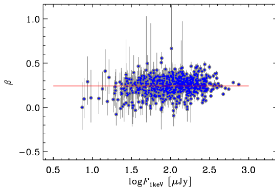
Figure 10. The behaviour of the \alpha (left-hand panel) and \beta (right-hand panel) parameters of the log-parabola model applied to the XRT spectra of Mrk 421 as a function of the unabsorbed flux density at 1 keV. The solid lines represent linear fits to the data.
