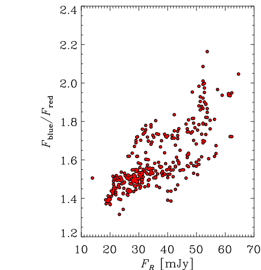
Figure 21. The Mrk 421 optical colour ('blue' to 'red' flux ratio) as a function of the source brightness (observed R -band flux density in mJy).
