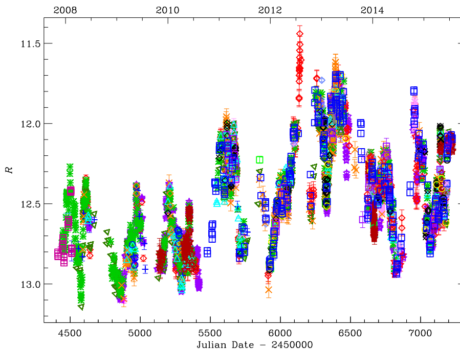
Figure 1. Optical light curve of Mrk 421 built with data from the GASP-WEBT collaboration and Steward Observatory in R band. Different colours and symbols highlight data from different telescopes. No correction for the host-galaxy contribution and Galactic extinction has been applied.
