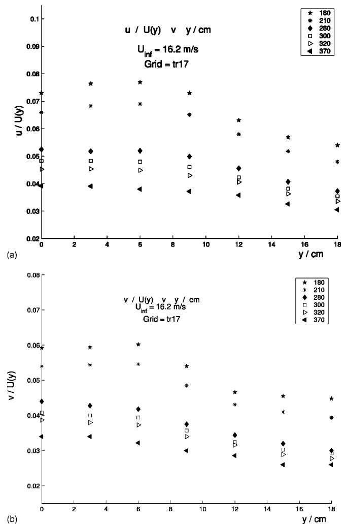
FIG. 4. Profiles of rms turbulence velocities at various streamwise locations between x=180 cm and =370 cm (given in cm in the inserts) downstream from the t_r=17.0 grid ( x_{\text{peak}} \approx 1.2 m) for U_\infty=16.2 m/s.
