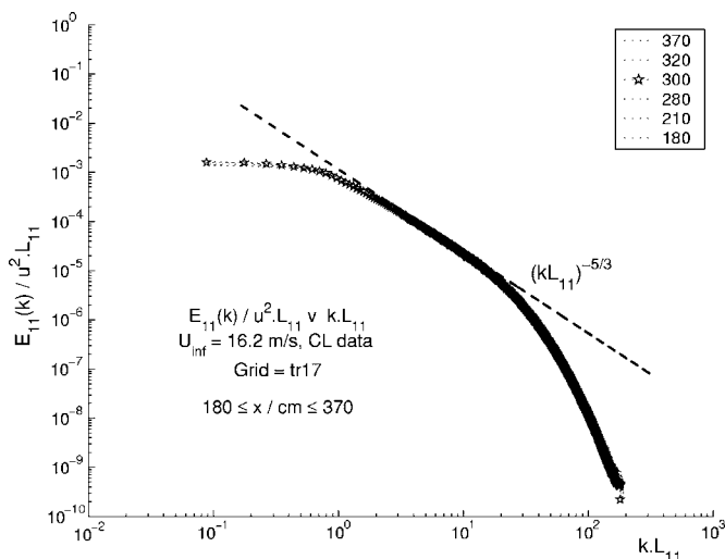
FIG. 12. E_{11}(k_1) / (u'^2 L_u) as a function of k_1 L_u for the t_r=17 grid at one of our highest values of U_\infty , U_\infty \approx 16 m/s, and at different values of x between x_{peak} and 3x_{peak} . The insert gives the values of x in cm corresponding to each spectral curve.
