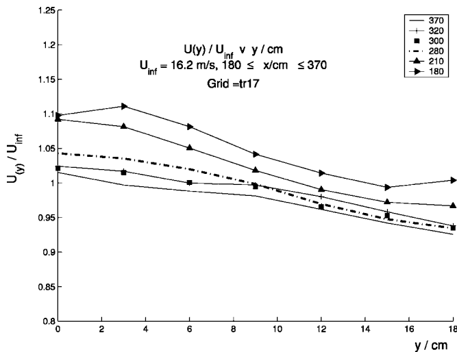
FIG. 3. Mean flow profiles at various streamwise locations between x=180 cm and =370 cm (given in cm in the insert) downstream from the t_r=17.0 grid ( x_{\text{peak}} \approx 1.2 m) for U_\infty=16.2 m/s. These profiles settle into a shape which varies little with x for x larger than about 2x_{\text{peak}} . In the region x \geq 2x_{\text{peak}} and -10 \text{ cm} \leq y \leq 10 \text{ cm} (note that L_{\text{max}}/2 \approx 12 cm), these profiles are approximately homogeneous.
