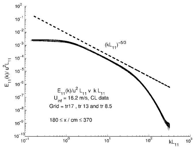
FIG. 14. E_{11}(k_1) / (u'^2 L_u) as a function of k_1 L_u for all three grids at one of our highest values of U_\infty , U_\infty \approx 16 m/s, and at the following values of x all larger than x_{peak} : x=1.8 m, 2.1 m, 2.8 m, 3.0 m, 3.2 m, and 3.7 m for t_r=17 where x_{peak} \approx 1.2 m; x=2.8 m, 3.0 m, 3.2 m, and 3.7 m for t_r=13 where x_{peak} \approx 1.45 m; x=3.2 m and 3.7 m for t_r=8.5 where x_{peak} \approx 1.8 m.
