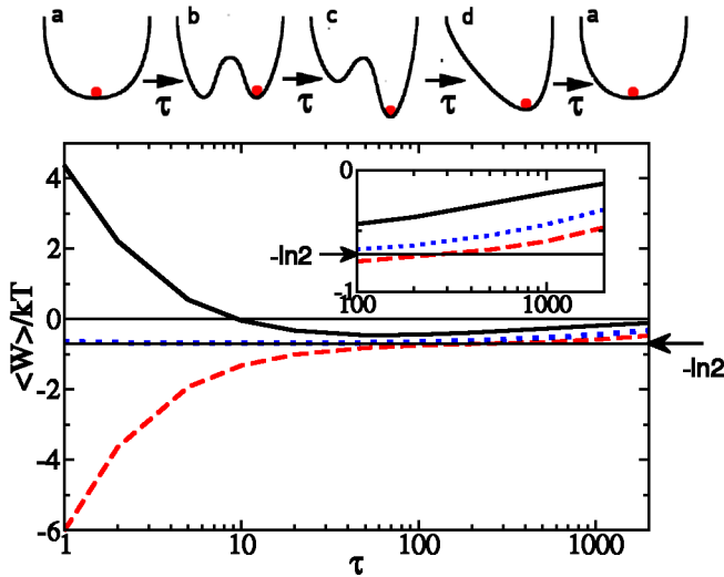
FIG. 3 (color online). Top: Cyclic variation of a model potential. The arrows indicate the forward protocol corresponding to the Szilard engine. The backward process is a model for recording and erasing information. Bottom: Partitioned average work as a function of processing time \tau : \langle W \rangle_R (solid line) and -\langle \tilde{W} \rangle_R (dashed line). The bound (8) using the coarse-grained distribution is shown by the dotted line.
