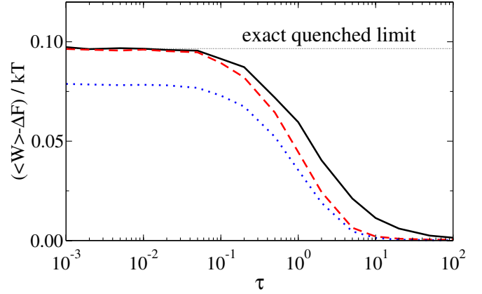
FIG. 2 (color online). Dissipation of Brownian particles in a harmonic potential with spring constant varying from \kappa = 2 to \kappa' = 1 during a time interval \tau . The solid line is dissipative work directly obtained from simulation. Dashed and dotted lines indicate the lower bound of the dissipative work estimated from the relative entropy.
