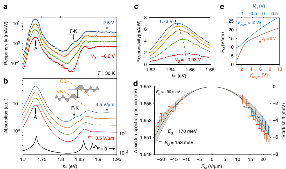
Fig. 2 Electroabsorption and Stark effect in monolayer WSe 2 p-n junctions. a Responsivity (PC/P) spectra measured at the p-n junction of device 3 (Supplementary Fig. 2) for various V_B , with a laser power P = 1 \mu\text{W} and T = 30 \text{ K} . The spectra are vertically shifted (by a factor of 1.5) for clarity. b Absorption spectra calculated using a Wannier-Mott exciton model at different in-plane electric fields F . The solid colored lines (left axis) were calculated with a phenomenological line shape broadening of 15 meV, while the black solid line (right axis) was calculated without broadening. All spectra are vertically shifted for clarity. Inset: Schematics illustrating the sub-bandgap, field-induced absorption increase due to the Franz-Keldysh (F-K) effect. The application of an in-plane field tilts the conduction (CB) and valence band (VB) of the semiconductor (orange lines) and allows the wave functions of the free electrons and holes (gray shaded curves) to leak into the bandgap, which results in an increase of the sub-bandgap absorption (dotted arrow). c Responsivity spectra (around the A exciton) measured on device 1 (shown in Fig. 1c) at various V_B , with a laser power P = 0.5 \mu\text{W} , V_{\text{asym}} = 10 \text{ V} and at room temperature. d Position of the A exciton as a function of the calculated F_M for the same values of V_{\text{asym}} and V_B as the one shown in e . Orange data points correspond to different values of V_{\text{asym}} at V_B = 0 \text{ V} , while blue data points represent different values of V_B at V_{\text{asym}} = 10 \text{ V} . Error bars correspond to the spectral resolution of our measurements. The calculated Stark shifts (right axis) induced by the F_M are represented by the black solid line ( E_B = 170 \text{ meV} ) and the gray shaded curves ( E_B = 153 and 190 \text{ meV} ). The latter values represent the uncertainty bounds of E_B arising from the uncertainty (95% confidence interval) in the measured polarizability. e Maximum in-plane electric field F_M calculated as a function of V_{\text{asym}} (with V_B = 0 \text{ V} , solid orange line) and as a function of V_B (with V_{\text{asym}} = 10 \text{ V} , solid blue line).
