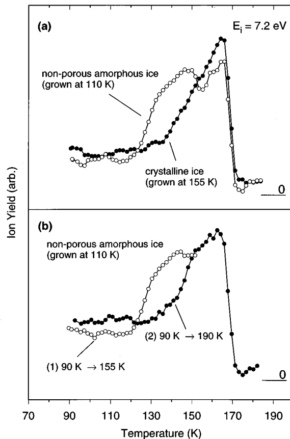
FIG. 9. (a) D^- signal vs temperature (90 \rightarrow 190 K, at 8 K/min), collected with E_i=7.2 \text{ eV} from 60-bilayer nonporous amorphous and crystalline ice films. (b) D^- signal vs temperature (90 \rightarrow 155 \rightarrow 90 \rightarrow 190 K), collected from a 60-bilayer nonporous amorphous ice film, using the same incident electron energy. For clarity, the first part of the temperature ramp (90 \rightarrow 155 K) is shown as open circles and the final part (90 \rightarrow 190 K) is shown as filled circles. The zeroes for the D^- data are indicated in the figure.
