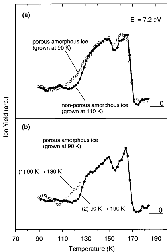
FIG. 8. (a) D^- signal vs temperature (90 \rightarrow 190 K, at 8 K/min), collected with E_i=7.2 \text{ eV} from 60-bilayer porous and nonporous amorphous ice films. (b) D^- signal vs temperature (90 \rightarrow 130 \rightarrow 90 \rightarrow 190 K), collected from a 60-bilayer porous amorphous ice film, using the same incident electron energy. For clarity, the first part of the temperature ramp (90 \rightarrow 130 K) is shown as open circles and the final part (90 \rightarrow 190 K) is shown as filled circles. The zeroes for the D^- data are indicated in the figure.
