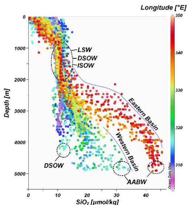
Fig. 4. Silicate profiles of the subpolar North Atlantic during the years 1996 to 2003. The depth range from 1000 m to 2200 m reflects Labrador Sea Water [LSW] in the Labrador and the West European Basin, Denmark Strait Overflow Water [DSOW] in the Reykjanes Basin, and Iceland Scotland Overflow Water [ISOW] in the Iceland Basin.
