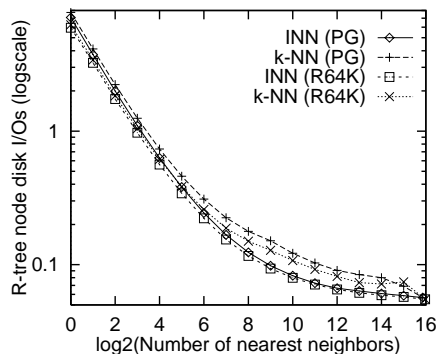
Fig. 21. R-tree node disk I/O per neighbor for k -nearest neighbor query.
