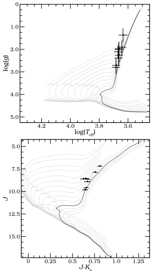
Fig. 8. Bottom: CMD of M67 giants on top of theoretical solar-metallicity Y^2 isochrones, with the 4 Gyr isochrone in black. The isochrones are spaced logarithmically in age between 0.01 to 15 Gyr. Horizontal lines indicate 1\sigma uncertainties in (J - K_s) and the uncertainties in the vertical direction are smaller than the size of the data-point. Top: Similar to top panel, except now for \log(g) versus \log(T_{\text{eff}}) .
