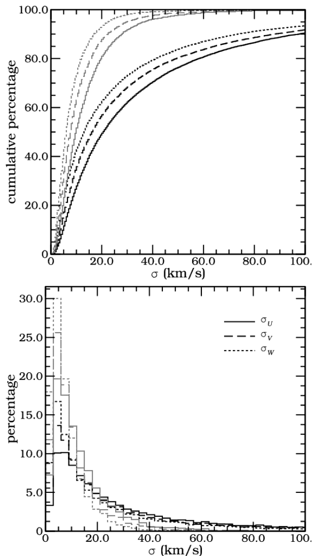
Fig. 9. Distribution of uncertainties for velocity components U (solid line), V (dashed line) and W (dotted line) velocities. This corresponds to the clean sample of 16146 stars (see §3.2). The black line includes all the stars, while the grey line shows the distribution for main-sequence stars (defined here as those with \log(g) > 4 ).
