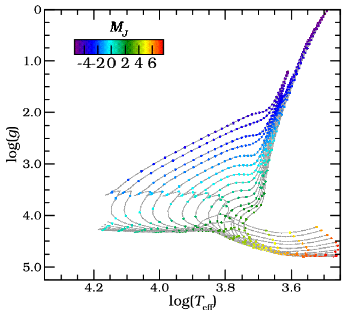
Fig. 1. \log(g) versus \log(T_{\text{eff}}) plot for isochrones from 0.01-15 Gyr spaced logarithmically, for [\text{M}/\text{H}] = 0 and [\alpha/\text{Fe}] = 0 . Colour indicates the absolute magnitude in the J band.
