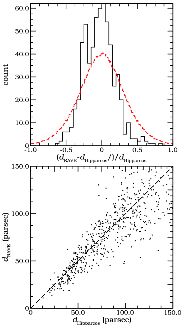
Fig. 6. Bottom: Distance from our method versus Hipparcos distance, the dashed line corresponds to equal distances. Top: Histogram of relative distance differences between our distance and that of Hipparcos. The dashed line shows the expected distribution given the quoted errors from our method and Hipparcos. Note that the observed distribution is narrower, indicating that our errors are probably overestimated for these stars (see §3.3.1).
