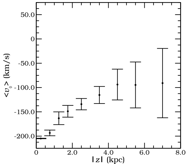
Fig. 12. Rotational velocity as a function of |z| for the high-quality subset of 5 020 stars (see §4). The error bars indicate 1\sigma uncertainty in the means. Note that the LSR has been assumed to move with v_\phi = -220 \text{ km s}^{-1} .
