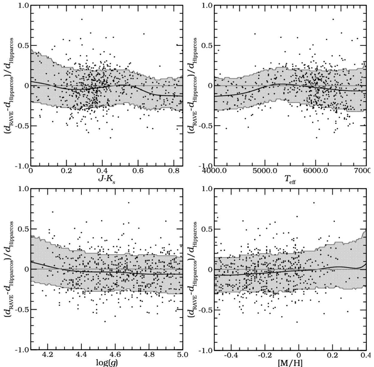
Fig. 7. Relative offset in distance from our method vs the trigonometric parallax determination from Hipparcos, as function of \log(g) , [M/H] , (J - K_s) and T_{\text{eff}} . We include a running mean and dispersion.
