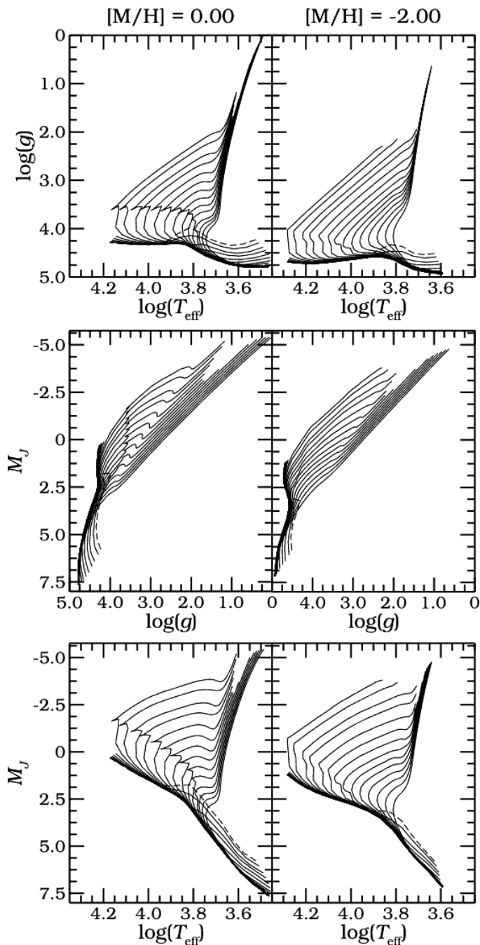
Fig. 2. Isochrones for [\alpha/\text{Fe}] = 0 , [M/H] = 0 (left column) and [M/H] = -2 (right column), ages ranging from 0.01-15 Gyr spaced logarithmically. The dashed line indicates the youngest (0.01 Gyr) isochrone. Top row: Similar to Fig. 1, shown for completeness. Middle row: M_J is best restricted by \log(g) for RGB stars. Bottom row: M_J is best restricted by T_{\text{eff}} for main-sequence stars.
