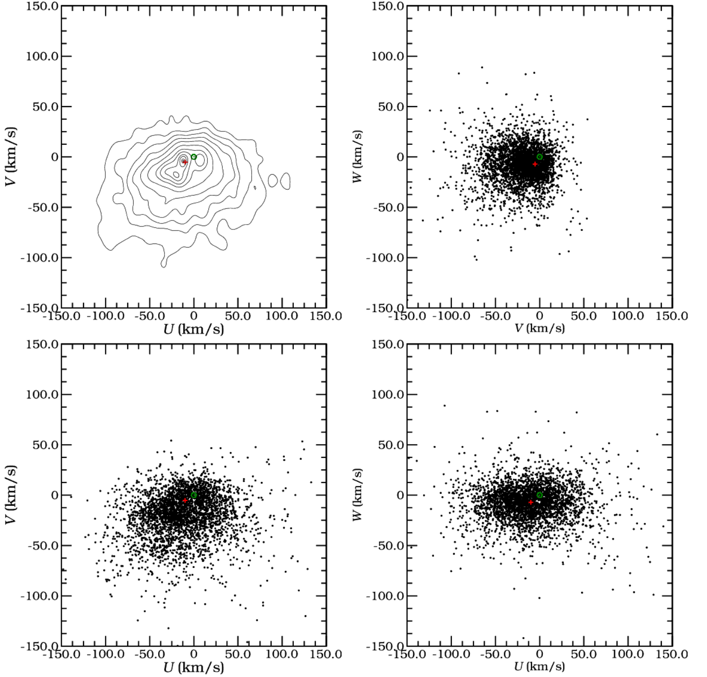
Fig. 14. The UV , UW and VW velocity distributions for the high-quality volume-limited sample of 3249 stars (see §4). The upper-left panel shows isodensity contours for the UV plane, where the contours contain 2, 6, 12, 21, 33, 50, 68, 80, 90, 99 and 99.9 percent of the stars. The red + symbol marks the LSR (Dehnen & Binney 1998) and the green \odot symbol marks the solar velocity (0, 0).
