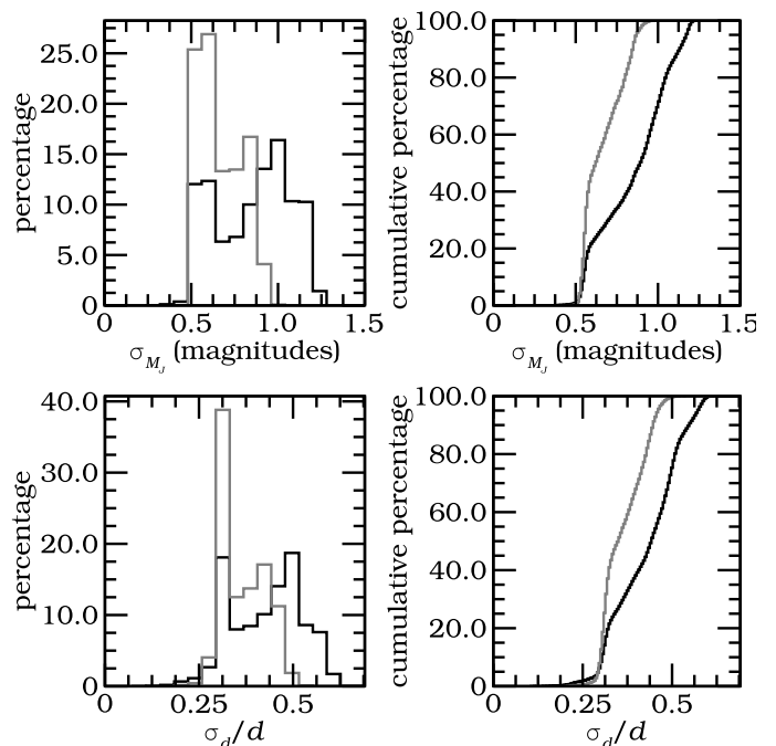
Fig. 4. Error distribution (left) and cumulative plot (right) for M_J (top) and distance (bottom). These distributions are for the clean sample of 16 146 stars (see §3.2). The black line includes all the stars, while the grey line shows the distribution for main-sequence stars (defined here as those with \log(g) > 4 ).
