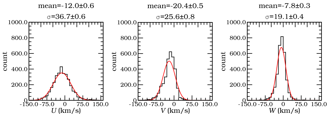
Fig. 13. Velocity distributions for the U , V and W components (histogram) and the best fit Gaussian (solid line) for high-quality volume-limited sample of 3249 stars (see §4). The velocity distributions for U and W are symmetric, showing a slight negative mean U and W owing to the solar motion with respect to the LSR. As expected, the V component shows a slight asymmetry, having a longer tail towards the slower rotating stars.
