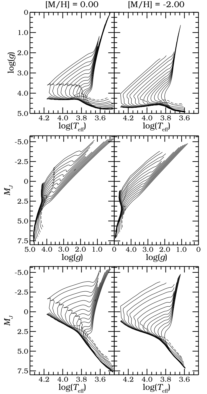
Fig. 2. Isochrones for [\alpha/Fe] = 0 , [M/H] = 0 (left column) and [M/H] = -2 (right column), ages ranging from 0.01–15 Gyr spaced logarithmically. The dashed line indicates the youngest (0.01 Gyr) isochrone. Top row: similar to Fig. 1, shown for completeness. Middle row: M_J is best restricted by \log(g) for RGB stars. Bottom row: M_J is best restricted by T_{\text{eff}} for main-sequence stars.
