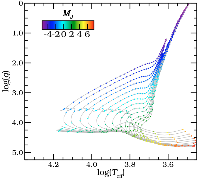
Fig. 1. \log(g) versus \log(T_{\text{eff}}) plot for isochrones from 0.01–15 Gyr spaced logarithmically, for [M/H] = 0 and [\alpha/Fe] = 0 . Colour indicates the absolute magnitude in the J band.
