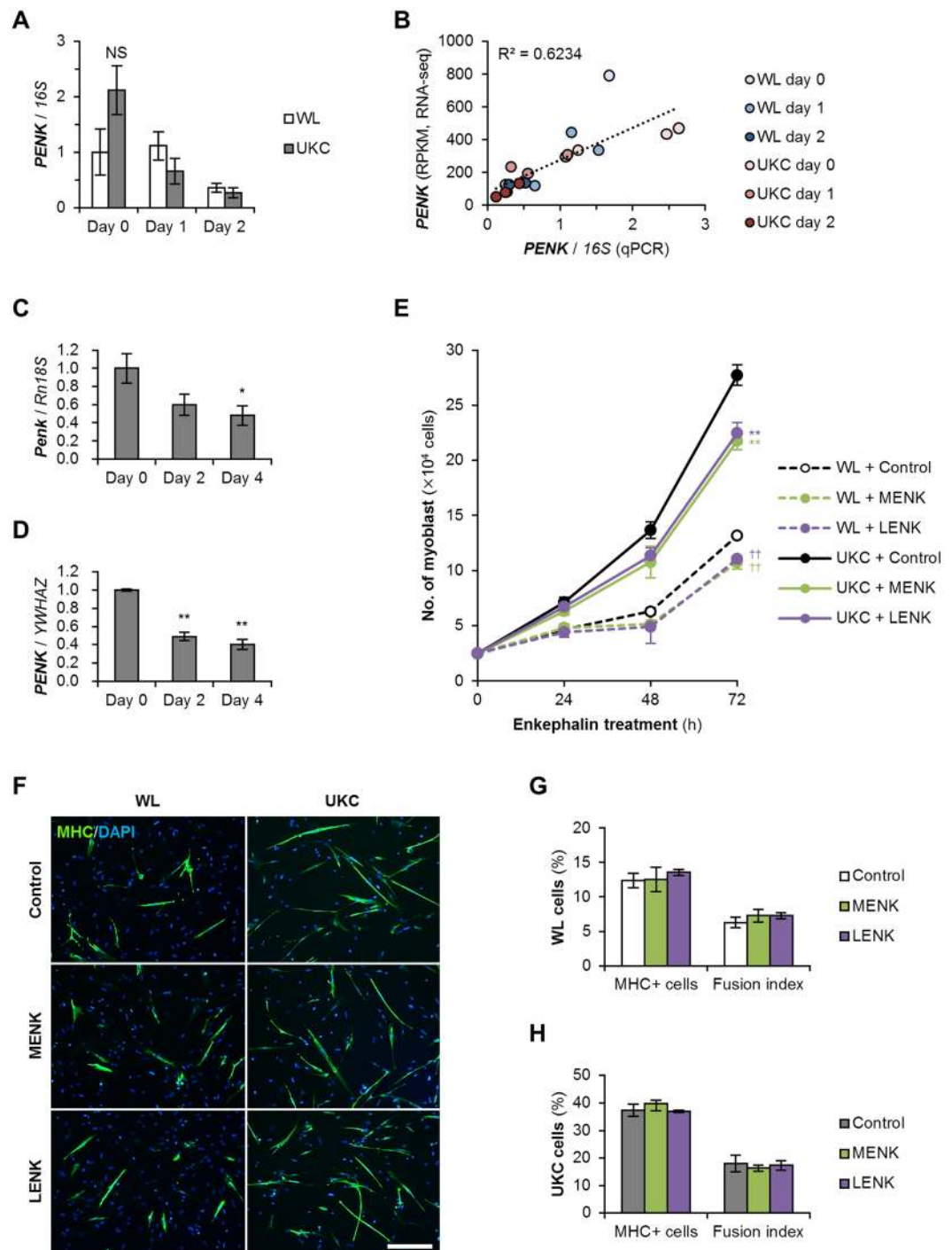
Figure 6. Enkephalin suppresses myoblast proliferation. (A) qPCR results of PENK gene transcription in the chicken myoblasts subjected to RNA-seq. NS, no significant difference vs WL (Student's t test at each time point). n = 3 . (B) Correlation of the chicken PENK gene transcription quantified by RNA-seq and qPCR (Pearson's correlation coefficient test). (C,D) qPCR results of pro-enkephalin gene transcription in murine (C) and human (D) myoblasts in DM. The mean value at day 0 was set at 1.0. * p < 0.05 , ** p < 0.01 vs day 0 (Williams' test). n = 3-4 . (E) Growth of WL and UKC myoblasts in GM with 1 \mu\text{M} MENK or LENK peptide. ** p < 0.01 vs control WL; ** p < 0.01 vs control UKC (Scheffe's F test at each time point). n = 4 . (F) MHC staining of WL and UKC myogenic cells in DM with 1 \mu\text{M} enkephalin at day 2. Scale bar, 200 \mu\text{m} . (G,H) The ratio of MHC + myocytes and fusion indexes of WL (G) and UKC (H) myogenic cells. No significant difference among control, MENK, and LENK samples in each group (Scheffe's F test). n = 4 .
