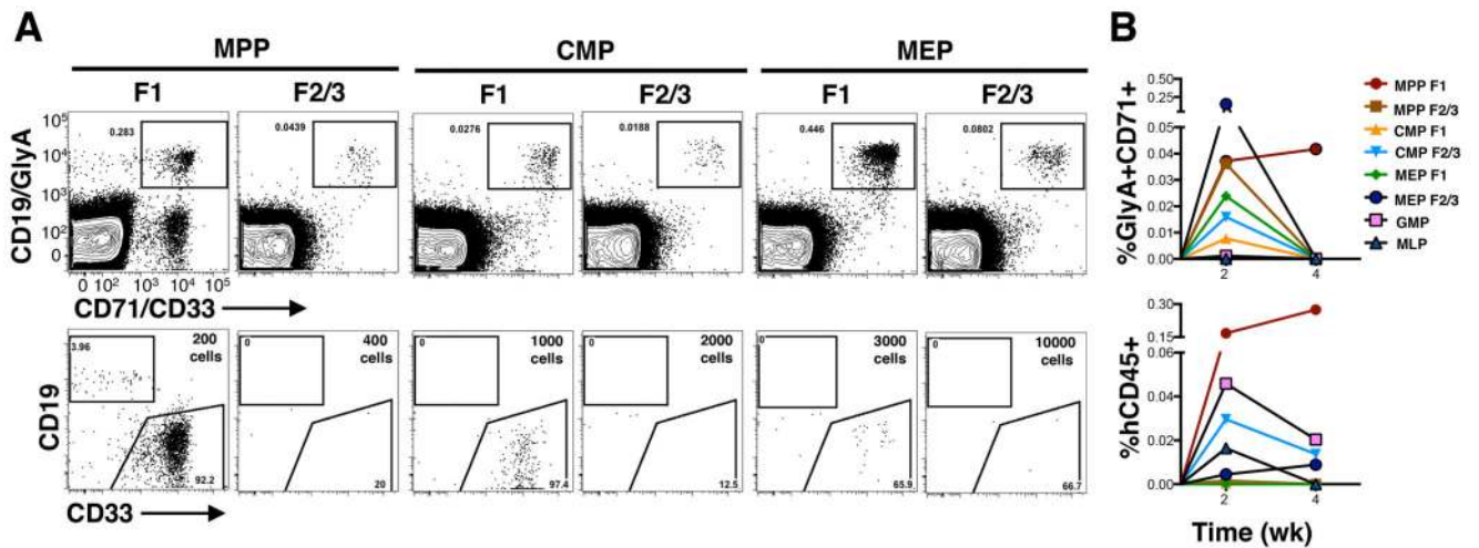
Figure 4. In vivo potential of progenitor subsets
