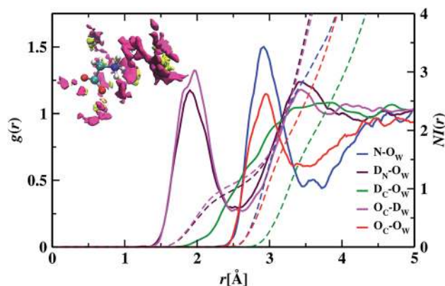
Fig. 1 In the glycine–water system, the solid lines blue, maroon, green, magenta, and red represent the radial distribution functions (RDFs) for N- O_w , D _N - O_w , D _C - O_w , O _C -D _w , and O _C - O_w pairs, respectively and the corresponding number integrals (NI) are shown with dashed lines. The SDF of oxygen and deuterium atoms are shown with magenta and yellow colored isosurfaces (isovalue = 78), respectively, in the upper part (inset figure).
