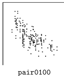
Figure 52: Scatter plots of pairs from D.37 . pair0100 : CPU cycle time \rightarrow Performance.
