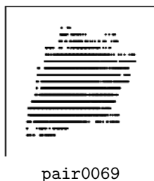
Figure 36: Scatter plots of pairs from D.20. pair0069: outside temperature \rightarrow inside temperature.
