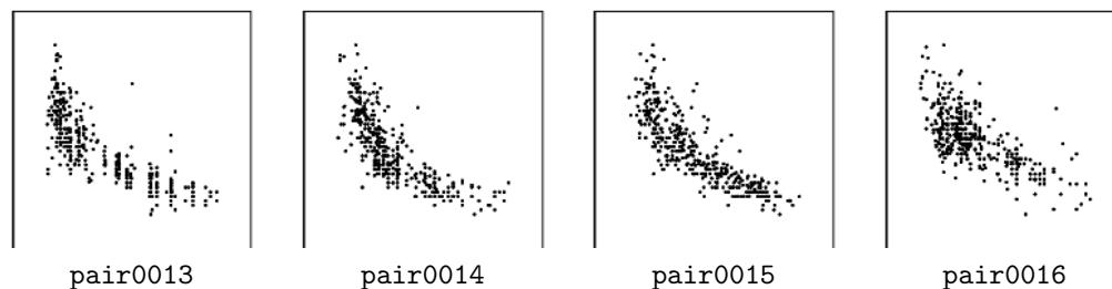
Figure 21: Scatter plots of pairs from D.4. pair0013: displacement \rightarrow fuel consumption, pair0014: horse power \rightarrow fuel consumption, pair0015: weight \rightarrow fuel consumption, pair0016: horsepower \rightarrow acceleration, pair0054: (displacement,horsepower,weight) \rightarrow (MPG,acceleration)
