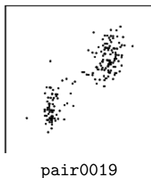
Figure 23: Scatter plots of pairs from D.6. pair0019: current duration \rightarrow next interval.
