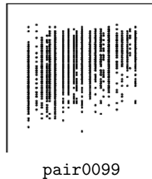
Figure 51: Scatter plots of pairs from D.36 . pair0099 : Social-economic status of family \rightarrow Language test score.
