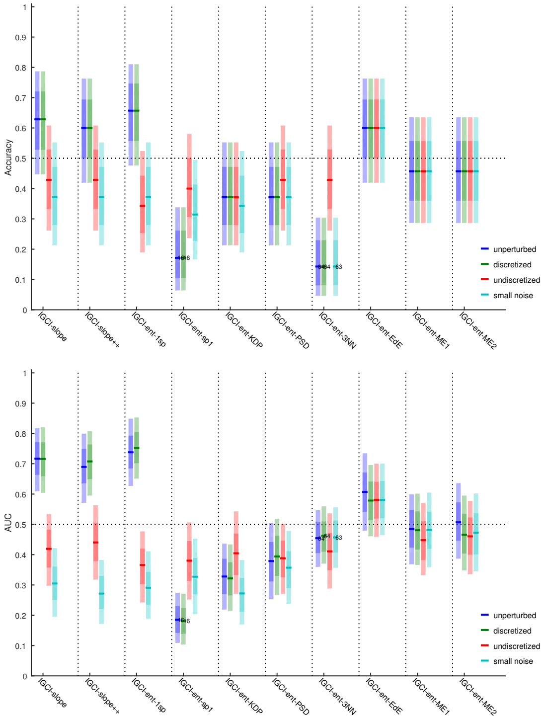
Figure 16: Accuracies (top) and AUCs (bottom) for various IGCI methods using the Gaussian base measure on different perturbations of the CEP benchmark data.
