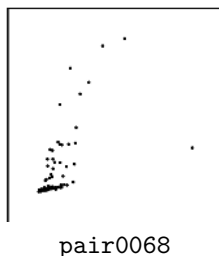
Figure 35: Scatter plots of pairs from D.19. pair0068: internet connections \rightarrow bytes transferred.
