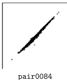
Figure 42: Scatter plots of pairs from D.27. pair0084 : population \rightarrow employment.
