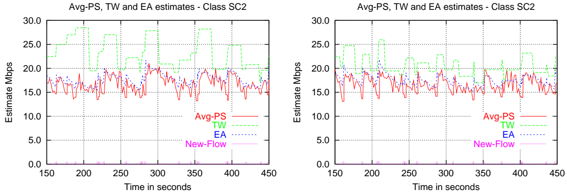
Figure 8. Estimation Mechanisms for ( T=10 ; S=2 ; \gamma = 0.25 ; flow(EXP,500kbps,i.a.t.=0.4s,h.t.=120s) (a) Reseting T (b) without Reseting T on Flow Admittance
