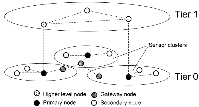
Figure 4. Two-tiered hierarchical WSN architecture (After Ref. [9]).
