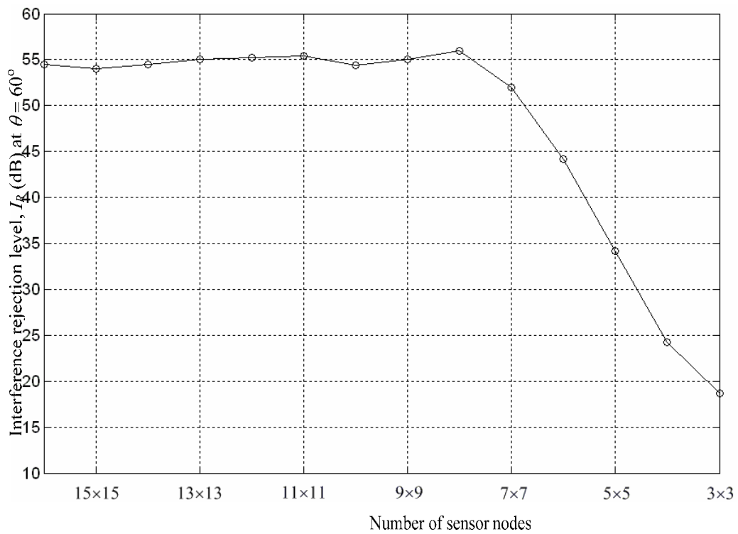
Figure 28. The interference rejection level as a function of the number of sensor nodes.
