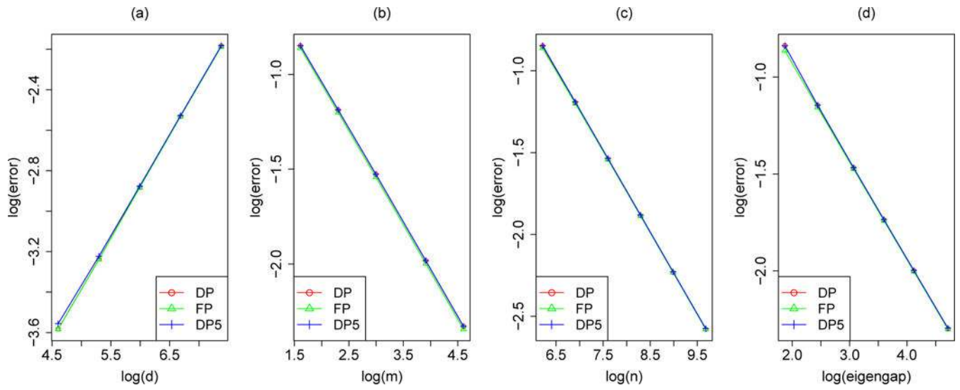
Figure 4: Comparison between DP, FP and DP5: (a) m = 20 , n = 2000 and \lambda = 50 ; (b) d = 1600 , n = 1000 and \lambda = 30 ; (c) d = 800 , m = 5 and \lambda = 30 ; (d) d = 1600 , m = 10 and n = 500 .
