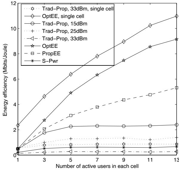
(a) Energy efficiency.
