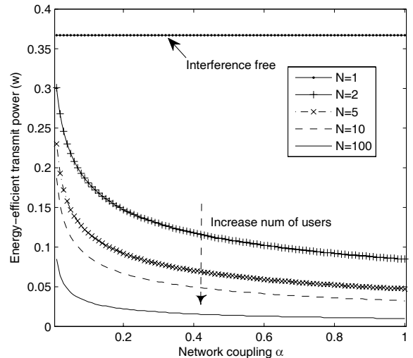
Fig. 2. Non-cooperative energy-efficient power optimization in the equilibrium ( P_c = 1, g = 1, \sigma^2 = 0.01 ).
