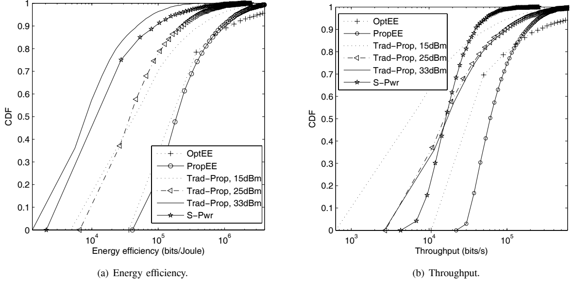
Fig. 4. Comparison of different schemes.
