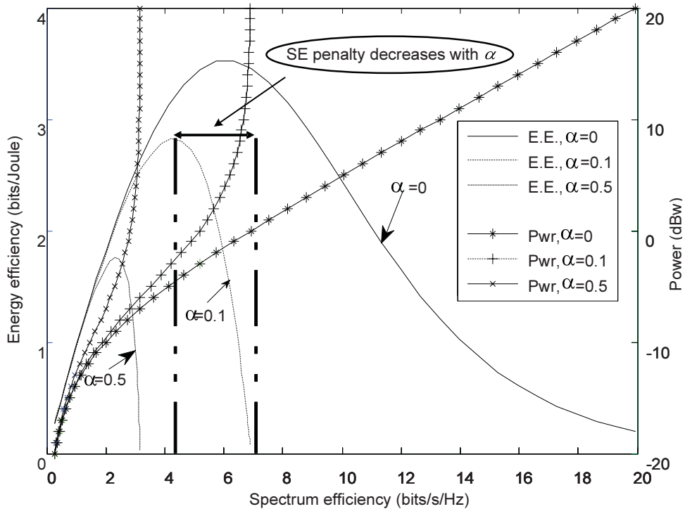
Fig. 1. Tradeoff of EE and SE with different interfering scenarios: left Y axis is for curves without markers and indicates the achieved EE while the SE is as in X axis; right Y axis is for curves with markers and indicates the required transmission power to achieve the spectral efficiency given in X axis. ( p_c = 1, g = 1, \sigma^2 = 0.01, N = 2 ).
