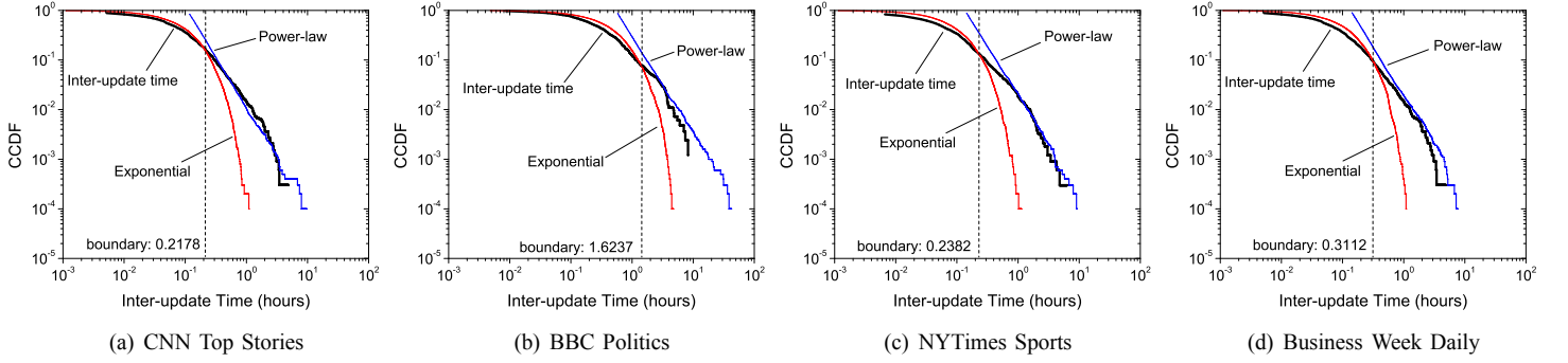
Fig. 3. CCDF of inter-refreshing time of individual RSS feeds
