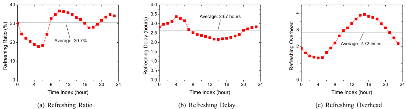
Fig. 14. Temporal variations of the performance of maintaining cache freshness
