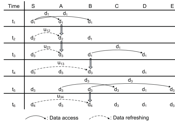
(b) Temporal sequence of data access and refreshing operations
