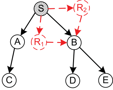
Fig. 8. Opportunistic replication of data updates
