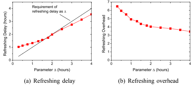
Fig. 12. Performance of maintaining cache freshness with different values of parameter \Delta and p = 60\%
