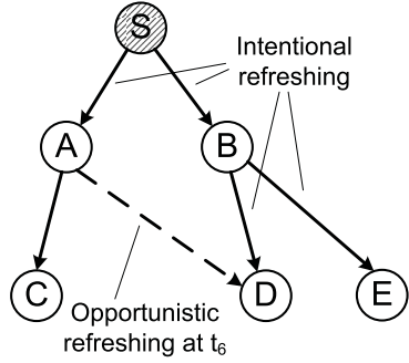
(a) Intentional and opportunistic refreshing
