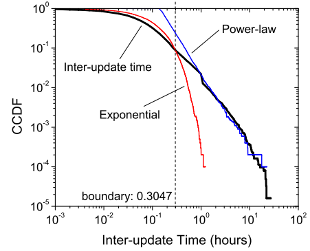
Fig. 4. Aggregate CCDF of the inter-refreshing time in log-log scale
