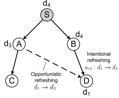
Fig. 9. Side-effect of opportunistic refreshing
