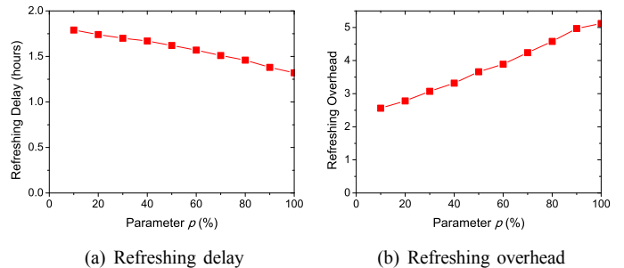
Fig. 13. Performance of maintaining cache freshness with different values of parameter p and \Delta = 1.5 hours
