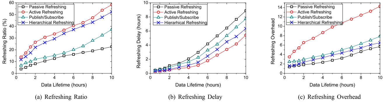
Fig. 11. Performance of maintaining cache freshness with varied lifetime of cached data
