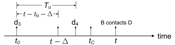
Fig. 7. Calculating the utility of data updates
