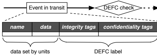
Fig. 5. An event with a DEFC label. DEFC labels are not controlled by units, but are used to enforce event flows.
