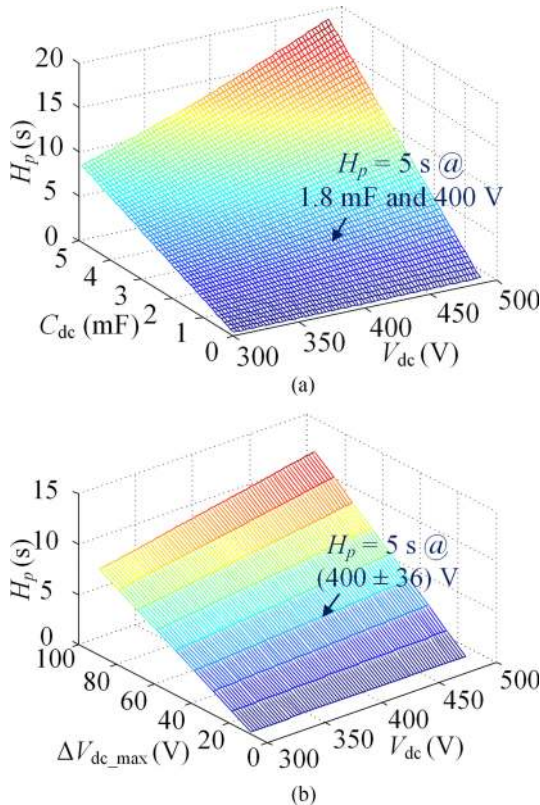
Fig. 9. Virtual inertia coefficient H_p versus C_{dc} , V_{dc} , and \Delta V_{dc,max} ( \Delta f_{r,max} = 0.2\text{Hz} , f_{ref} = 50\text{Hz} , and VA_{rated} = 1\text{kVA} ). (a) \Delta V_{dc,max}/V_{dc} = 0.15 . (b) C_{dc} = 2.82\text{mF} .
