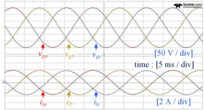
Fig. 15. Experimental waveforms of the grid voltages v_{gx} and load currents i_{lx} ( x = a, b, c ).
