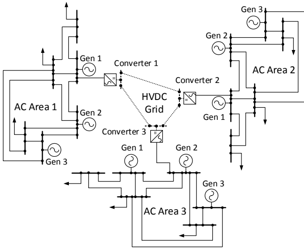
Figure 2. Test grid consisting of 3 AC areas, connected by an MTDC grid consisting of 3 converter stations and 3 DC lines.
