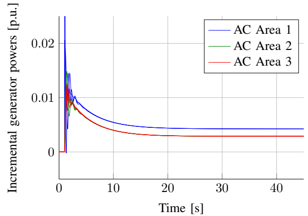
Figure 4. Incremental generator power levels.
