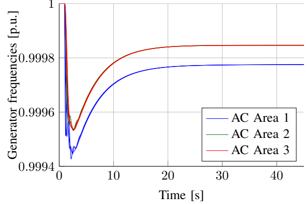
Figure 3. Frequencies of the generator areas.
