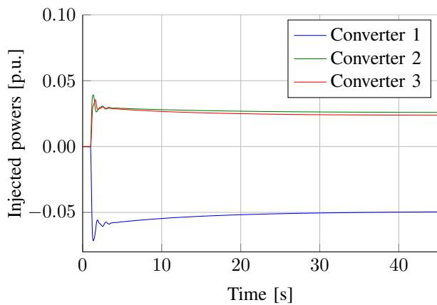
Figure 5. Injected power levels at the converters.
