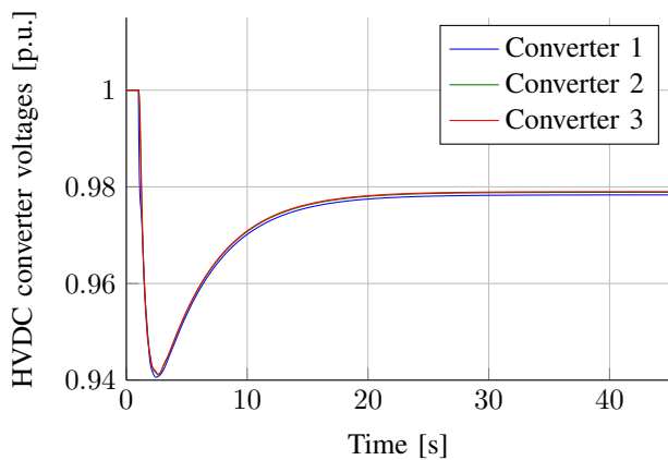
Figure 6. Voltages of the DC converters.
