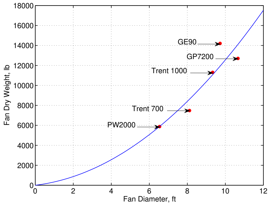
Figure 8: Estimated Fan Weight vs. Fan Diameter for Commercial Turbofan Engines
