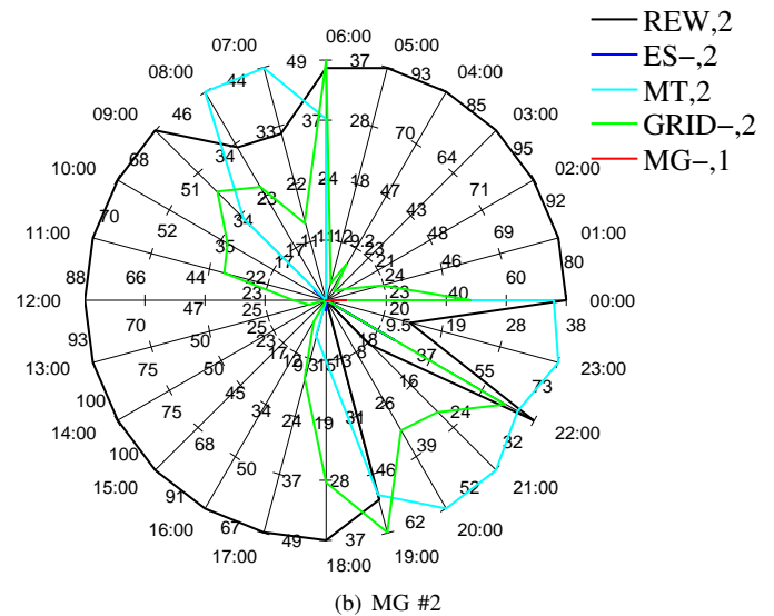
Fig. 11: Percentage of the electricity generation accounted by all DER resources in a) MG #1 b) MG #2
