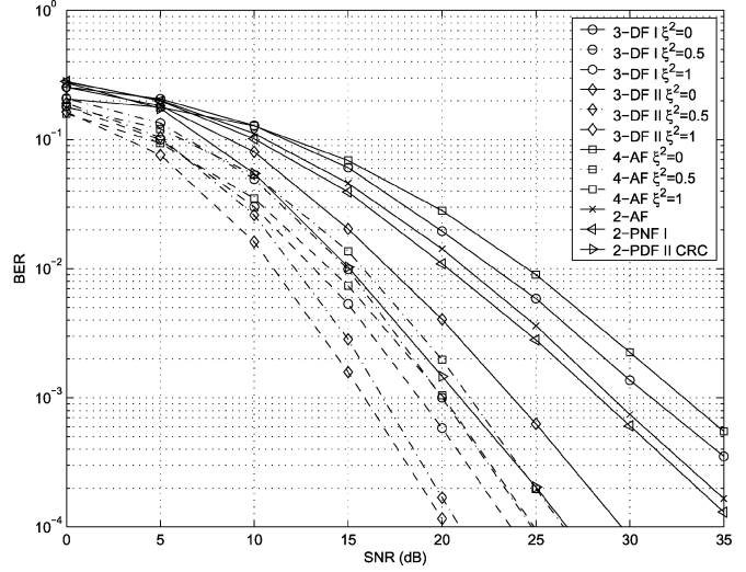
Fig. 6. Performance comparison of 2, 3, and four-time-slot protocols in a network with two relays when there is direct transmission between the two terminals. Two-time-slot protocols use 4-QAM, three-time-slot protocols use 8-QAM, and four-time-slot protocols use 16-QAM.
