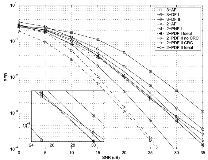
Fig. 4. Performance comparison of two-time-slot protocols and three-time-slot protocols in a network with two relays. two-time-slot protocols use 4-QAM and three-time-slot protocols use 8-QAM.
