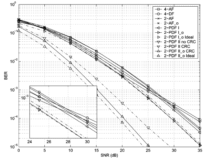
Fig. 3. Performance comparison of two-time-slot protocols and four-time-slot protocols in a network with two relays. two-time-slot protocols use BPSK and four-time-slot protocols use 4-QAM.
