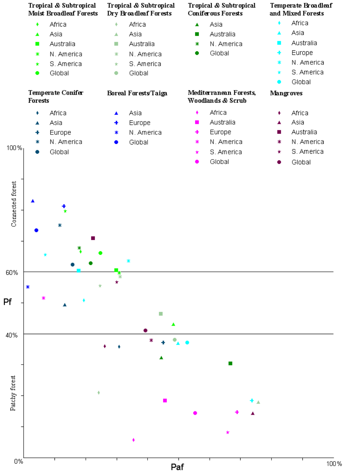
Fig. 3. Scatter plot of the proportion of forest ( P_f ) vs. anthropogenic fragmentation ( P_{fa} ) for each combination of continent and biome. The horizontal lines drawn at P_f = 40 and 60 represent possible thresholds of connectivity (see text). For a given value of P_{fa} , the relative value of P_f may help identify biomes and continents where anthropogenic fragmentation is more or less of an issue.
