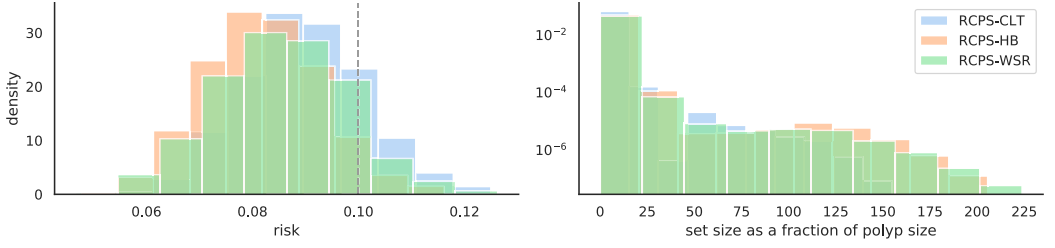
Fig. 13. Polyp segmentation results. The risk and normalized set size are plotted as histograms over different random splits of the polyp dataset, with parameters \alpha = 0.1 and \delta = 0.1 . For details, see Section 5.4.
