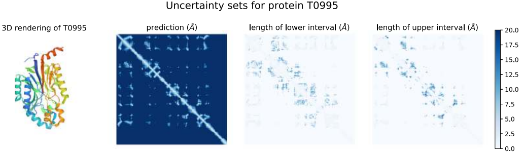
Fig. 14. Protein distograms. We show AlphaFold’s predicted distances between residues of protein T0995 along with prediction sets at \alpha = 2\text{\AA} and \delta = 0.1 . The prediction set for the whole protein is the union of distance intervals for each pair of residues, and the right two panels report the distance from the point prediction to the lower and upper endpoints for each of these intervals.
