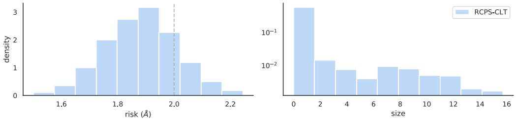
Fig. 15. Protein structure prediction results. The risk in \text{\AA} and interval size (pooling all entries of each distogram) in \text{\AA} are plotted as histograms, repeating for many random splits of the CASP-13 test-set.
