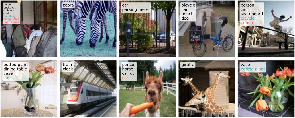
Fig. 8. Multi-label prediction set examples on MS COCO. Black classes are correctly identified (true positives), blue ones are spurious (false positives), and red ones are missed (false negatives).
