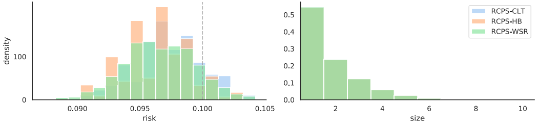
Fig. 7. Prediction set results on Imagenet. The risk and set sizes for an RCPS are plotted as histograms over 100 different random splits of Imagenet, with parameters \alpha = 0.1 and \delta = 0.1 . For details, see Section 5.1. The set sizes for all three methods overlap.
