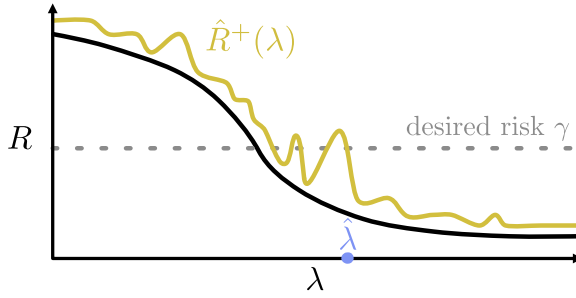
Fig. 3. Visualization of UCB calibration.
