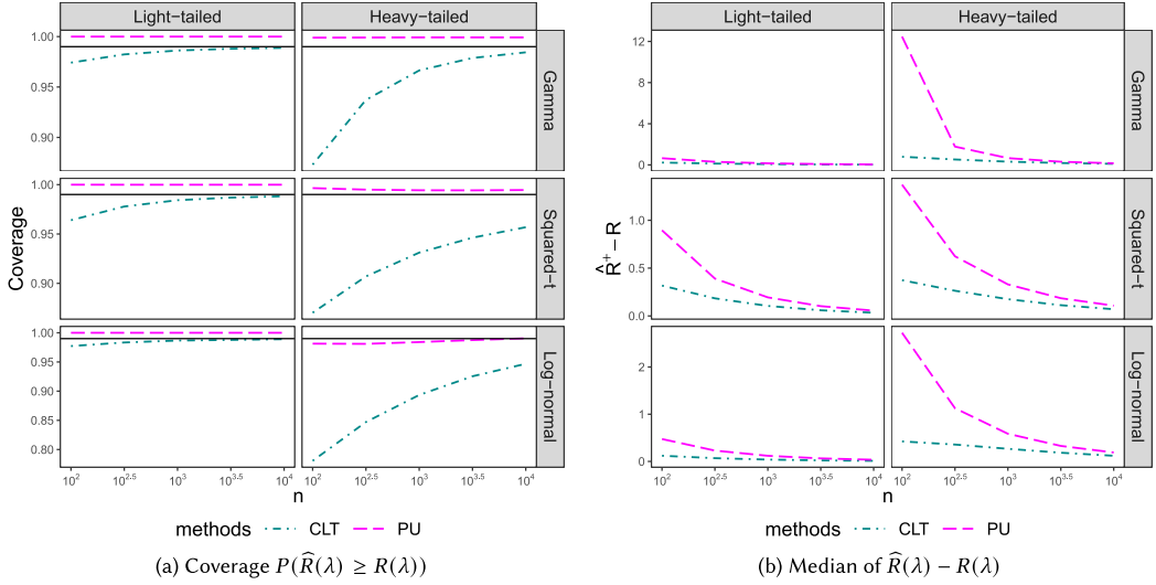
Fig. 18. Numerical evaluations of the PU bound (9) with the estimated coefficient of variation and the CLT bound (10), on a million independent samples of size n from each distribution in Table 1 with \delta = 0.01 . Each row corresponds to a type of distribution, and each column corresponds to a value of the mean.
