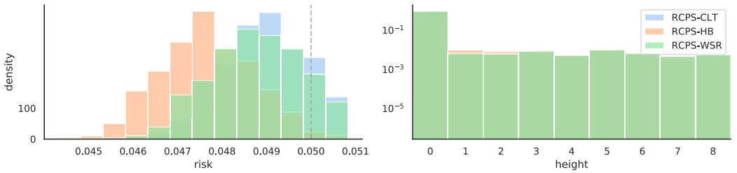
Fig. 11. The risk and height of RCPS for hierarchical classification. We show histograms of risk and height (distance from the leaf node) over 100 different random splits of the Imagenet dataset, with parameters \alpha = 0.05 and \delta = 0.1 . For details, see Section 5.3.
