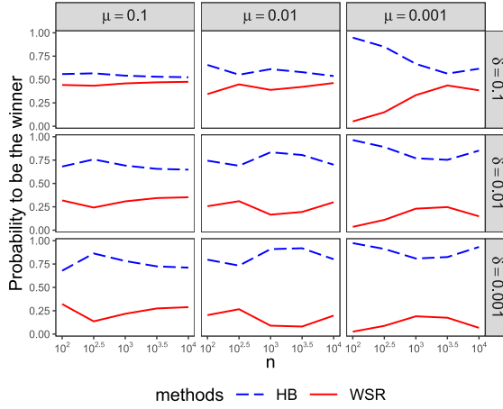
Fig. 20. Fraction of samples on which the HB bound or the WSR bound is the winner among the four bounds, excluding the CLT bound, for Bernoulli distributions. Each row corresponds to a level and each column corresponds to a value of mean.
