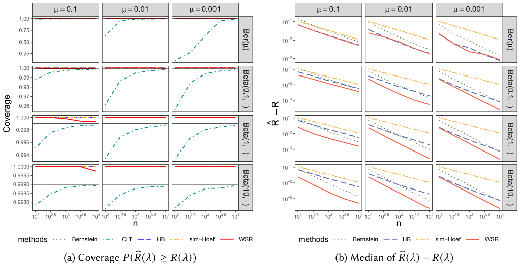
Fig. 17. Numerical evaluations of the simple Hoeffding bound (5), HB bound (7), empirical Bernstein bound (8), CLT bound (10), and WSR bound (Proposition 5) on a million independent samples of size n with \delta = 0.001 . Each row corresponds to a type of distribution, and each column corresponds to a value of the mean. The CLT bound is excluded in (b) because it does not achieve the target coverage in most of the cases.
