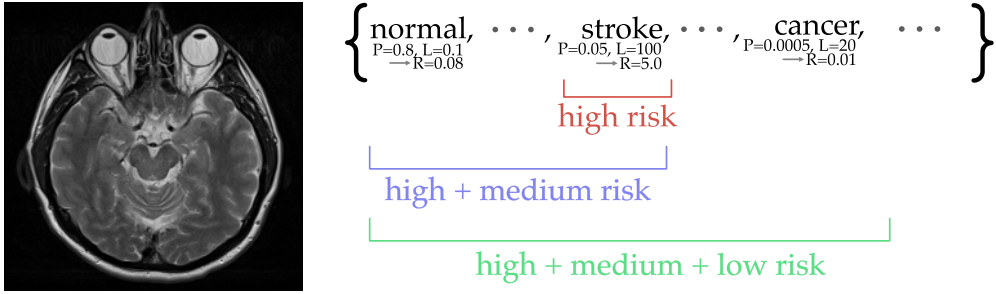
Fig. 1. A stylized example of risk-controlling prediction sets. Here, “P” gives the estimated probability for each class, the loss per class is labeled as “L,” and the loss times the probability is the estimated risk, labeled as “R.” The red, blue, and green brackets represent possible sets of labels that our procedure may output.
