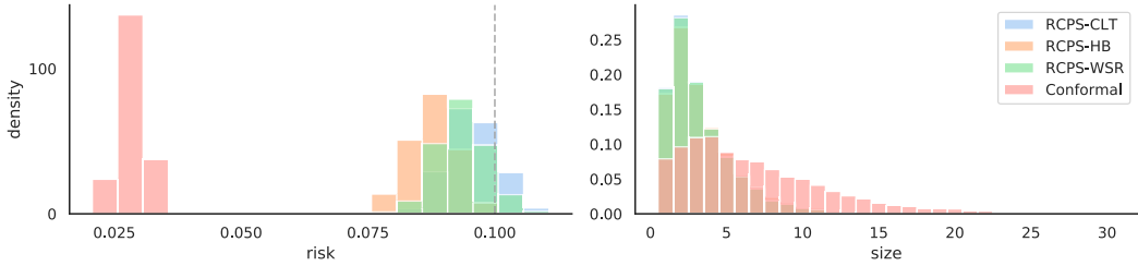
Fig. 9. Multi-label prediction set results on MS COCO. The risk and set sizes are plotted as histograms over 1,000 different random splits of MS COCO, with parameters \alpha = 0.1 and \delta = 0.1 . We also include a conformal baseline. For details, see Section 5.2.
