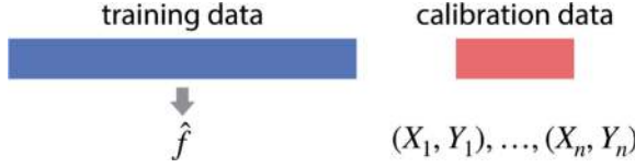
Fig. 2. Sample-splitting setup. The training data is used to fit a predictive model \hat{f} . The remaining data is used to calibrate a set-valued predictor (based on \hat{f} ) to control risk, as described in this work.
