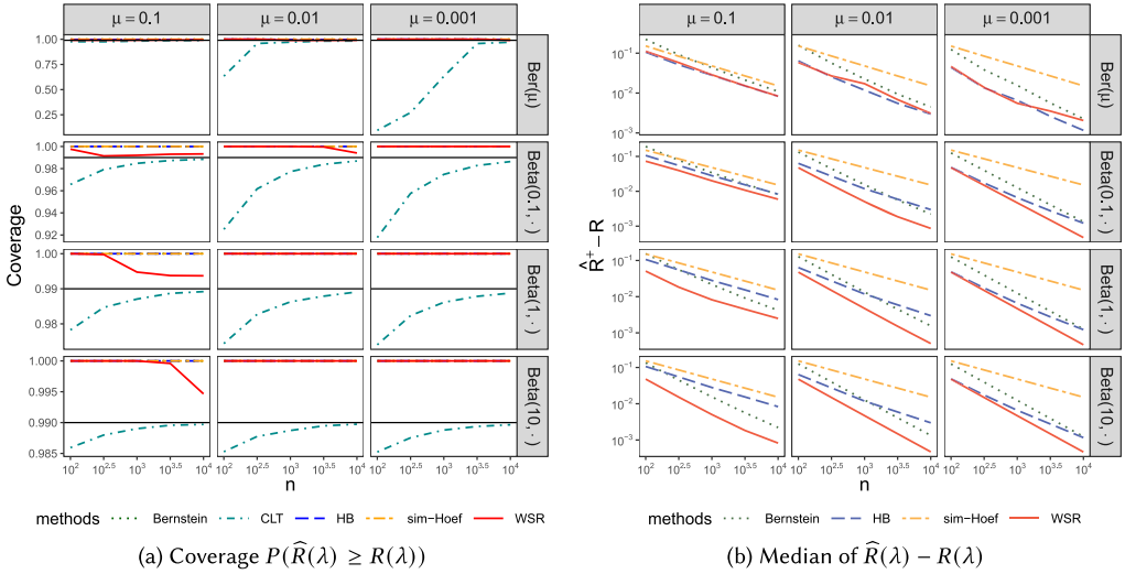
Fig. 16. Numerical evaluations of the simple Hoeffding bound (5), HB bound (7), empirical Bernstein bound (8), CLT bound (10), and WSR bound (Proposition 5) on a million independent samples of size n with \delta = 0.01 . Each row corresponds to a type of distribution, and each column corresponds to a value of the mean. The CLT bound is excluded in (b) because it does not achieve the target coverage in most of the cases.
