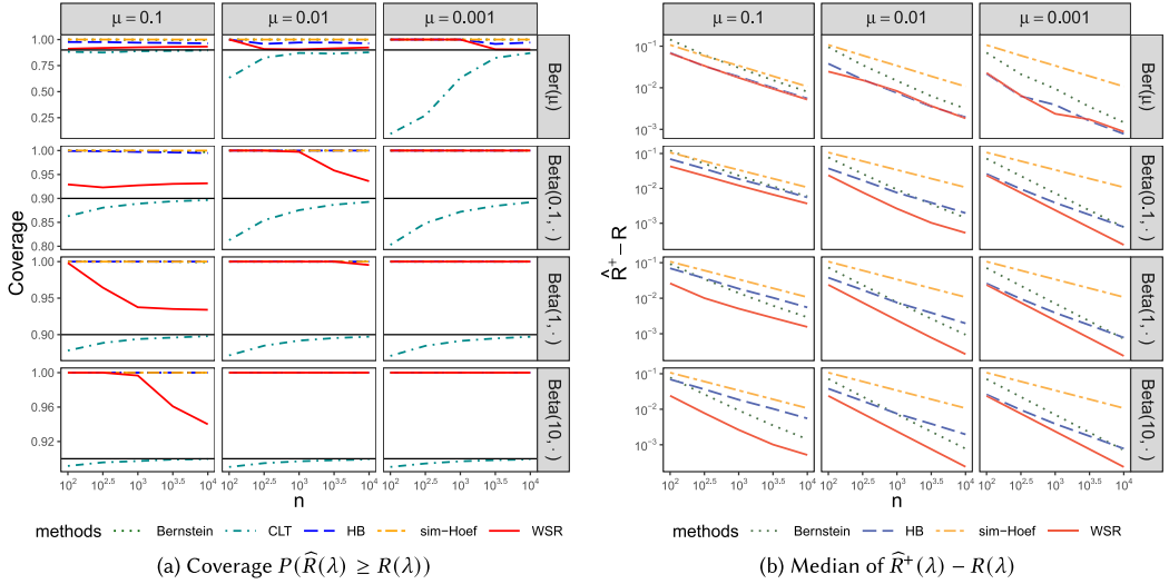
Fig. 4. Numerical evaluations of concentration results for bounded losses. We show the simple Hoeffding bound (5), HB bound (7), empirical Bernstein bound (8), CLT bound (10), and WSR bound (Proposition 5) with sample size n . Each row corresponds to a type of distribution and each column corresponds to a value of the mean. The CLT bound is excluded in (b), because it does not achieve the target coverage in most of the cases.
