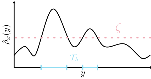
Fig. 6. Optimal prediction sets. In the special case where \hat{\rho}_x(y, \mathcal{S}) does not depend on \mathcal{S} , \mathcal{T}_\lambda(x) from Algorithm 1 is made up of the y \in \mathcal{Y} whose conditional risk density exceeds a threshold \zeta .
