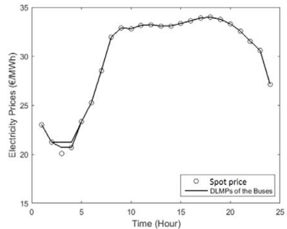
Fig. 9. DLMPs calculated with deterministic optimizations.
