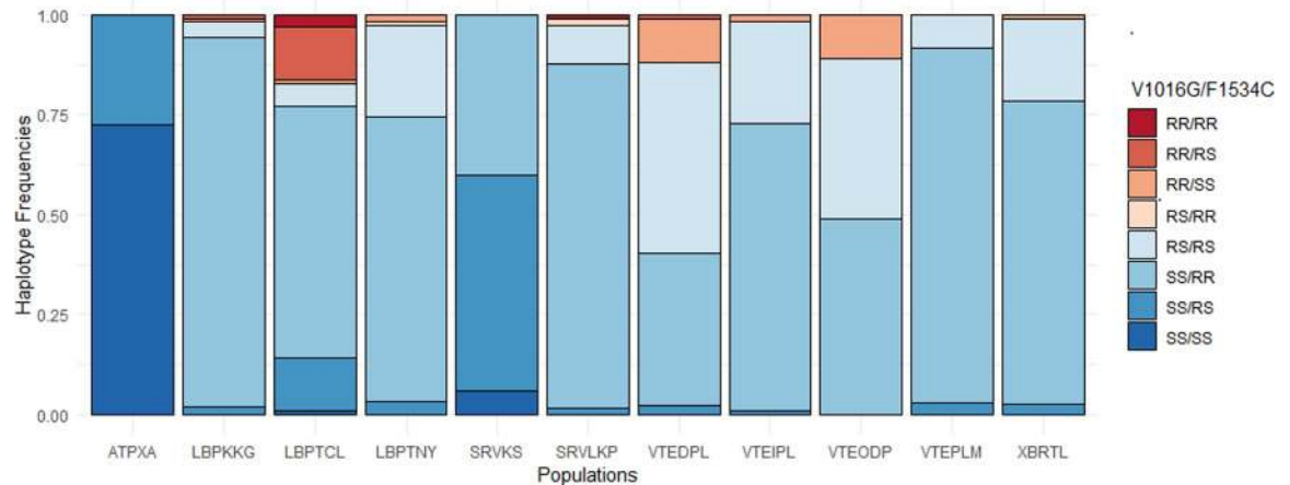
Fig 5. Haplotypes frequencies of V1016G and F1534C kdr mutations in Aedes aegypti populations from Laos.
