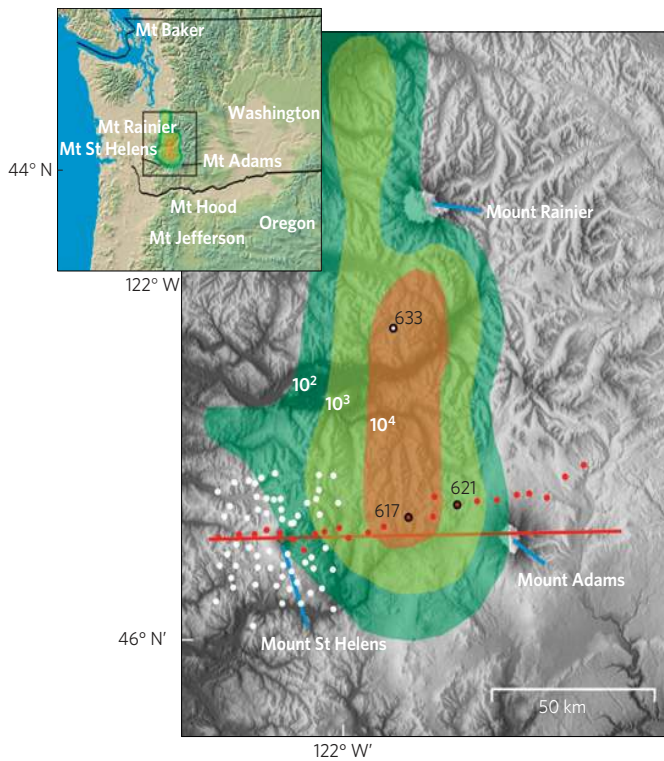
Figure 1 | Locations of magnetotelluric measurement sites, Mount St Helens and nearby Cascades volcanoes. The box drawn around Mounts St Helens and Adams in the inset map outlines the area of the magnetotelluric survey shown in the adjacent map. White and red dots show the locations of the magnetotelluric measurements; measurement sites shown in red were used for the phase-tensor pseudo-section (Fig. 3) and 2D inversion (Fig. 4a). The east–west line (red) shows the profile onto which these measurements were projected. The coloured area shows the region of high conductance 5 . The green-to-orange transition corresponds to the 3 \times 10^3 S contour in Fig. 2.
