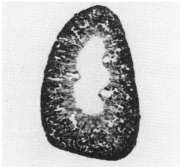
FIGURE 4. Detail (kidney) of whole-body autoradiogram from a mouse intravenously injected with ^{109}\text{CdBP} and killed after 4 hr.
