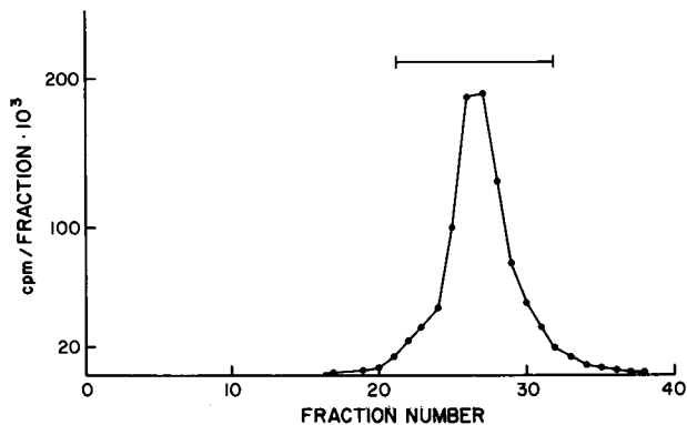
FIGURE 2. G-75 Sephadex chromatography of ^{109}\text{CdMT-1} . Column dimensions, 365 × 25 mm. Elution with 0.1M Tris buffer - 0.5M NaCl, pH 8.0, + 4°C. Fractions of 5 ml were collected at 14 ml/hr. Fractions 21-31 indicated by the bold line were concentrated, buffer concentration and pH adjusted to physiological values (0.9% NaCl, pH 7.2), and injected intravenously in mice. Recovery of Cd, 98%.
