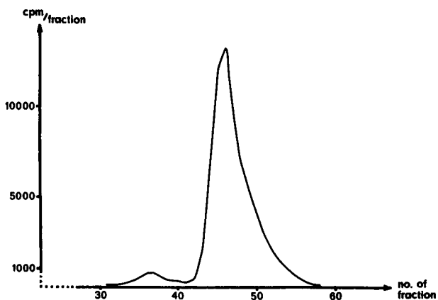
FIGURE 1. G-50 Sephadex chromatography of a sample of ^{109}\text{CdBP} . Column dimensions 885 × 25 mm. Elution with 0.01M Tris buffer - 0.05M NaCl, pH 8.0, + 8°C. Fractions of 5 ml were collected at 28 ml/hr. Recovery of Cd, 98%.
