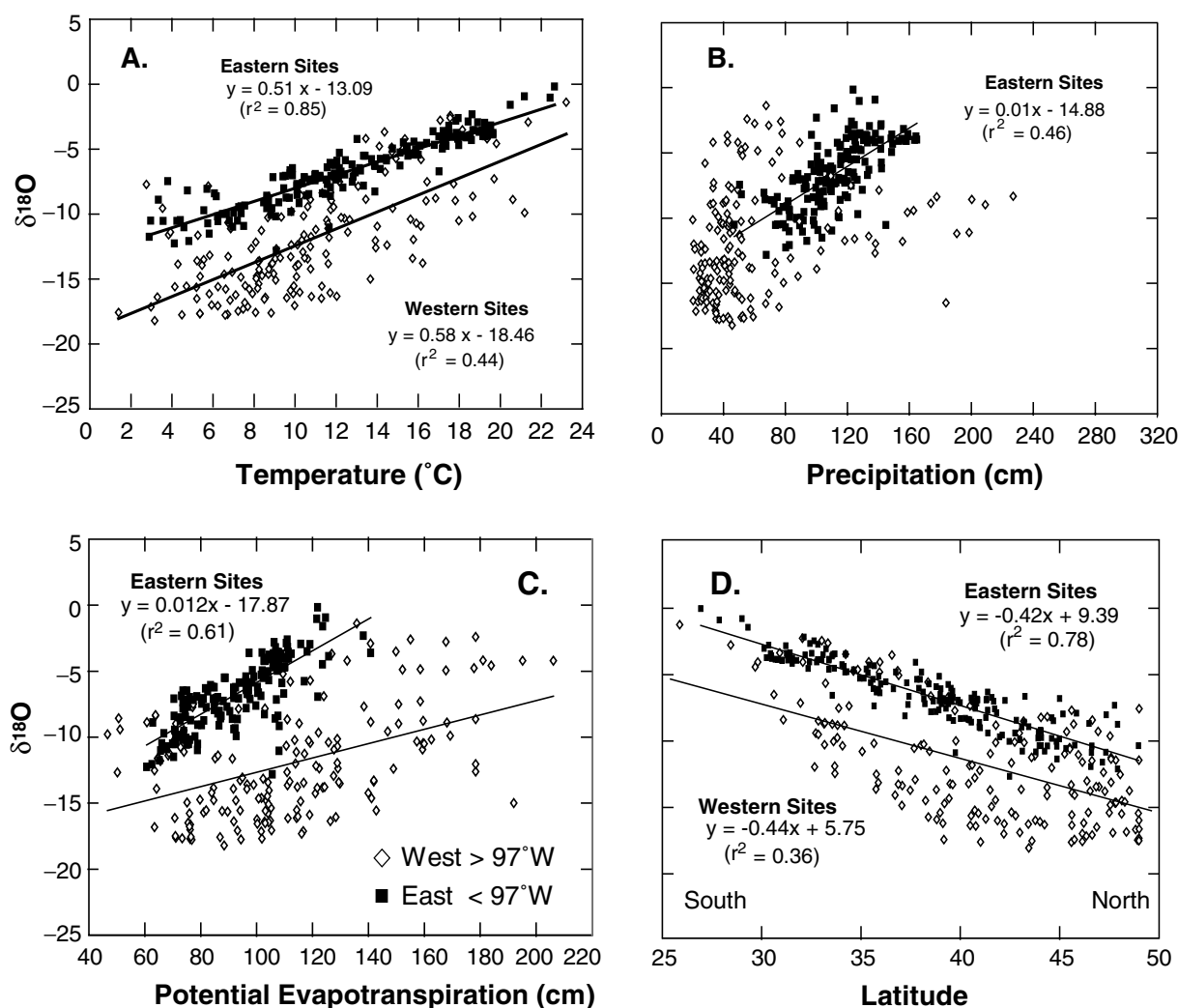
Figure 10. Relations between mean annual \delta^{18}\text{O} and (a) temperature ( ^{\circ}\text{C} ), (b) precipitation (cm), (c) mean PET (cm), and (d) latitude ( ^{\circ}\text{N} ). Temperature and precipitation data are means for 1961–90 (NOAA, 1999); PET data are from Farnsworth et al. (1982)
