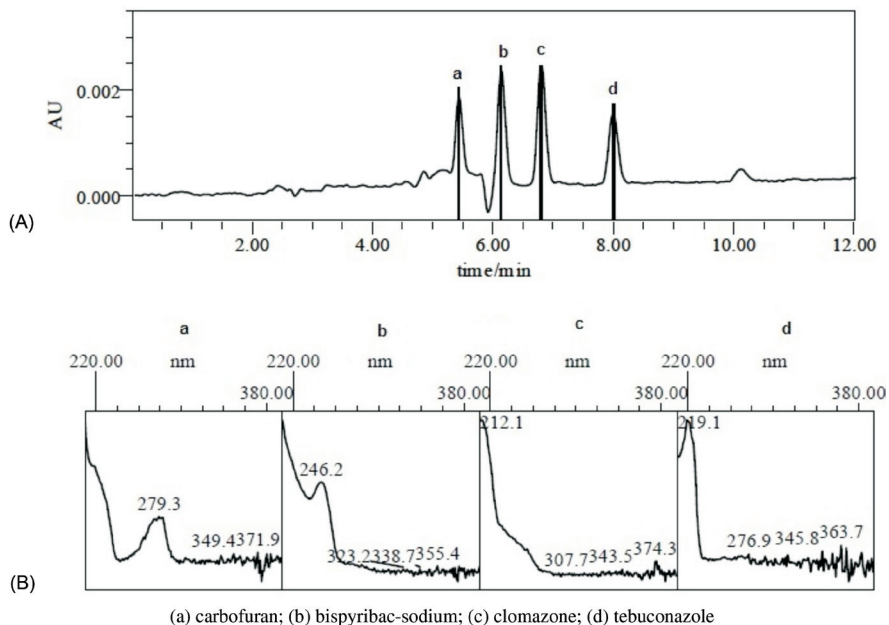
Figure 1. Chromatogram at LOQ concentration (A) and UV spectra (B). (HPLC conditions: monitoring at 220 nm; Synergi Fusion-RP 80A column; mobile phase acetonitrile/water (70:30 v/v) adjusted for pH 3.0 with H_3PO_4 (1:1 v/v) and flow rate of the 0.8 \text{ mL min}^{-1} ).
