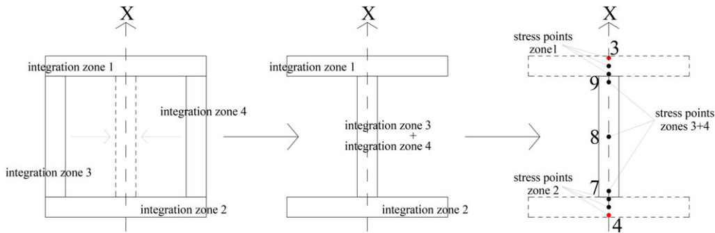
FIGURE 3 Conversion scheme box-to-I shape cross section of the core. Integration/stress points are depicted for each integration zone
