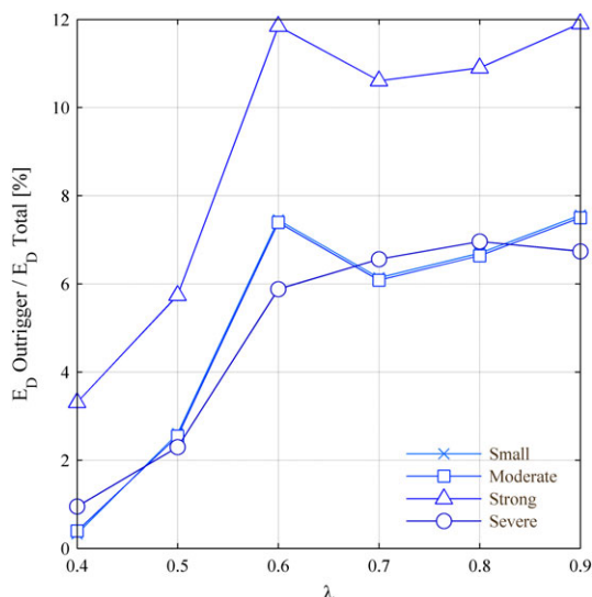
FIGURE 23 Damping energy (in %) dissipated only by the outriggers, under the combined influence of \lambda and different earthquake levels of 1940 El Centro earthquake; C_d = 1.18E + 05\text{kN-s/m} and \zeta = 2.0\%
