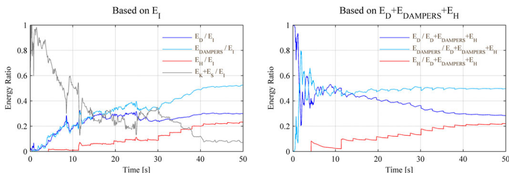
FIGURE 21 Energy ratios based on E_I and E_D + E_{dampers} + E_H , for the damped outrigger under strong earthquake level of 1940 El Centro earthquake; C_d = 1.18E + 05kN-s/m , \lambda = 0.7 and \zeta = 2.0\%
