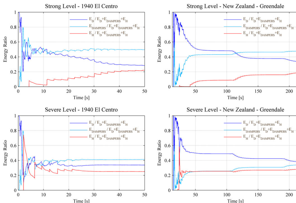
FIGURE 22 Energy ratios of the damped outrigger ( C_d = 1.18E + 05\text{kN}\cdot\text{s}/\text{m} , \lambda = 0.7 and \zeta = 2.0\% ), under strong and severe levels of 1940 El Centro and New Zealand–Greendale earthquakes
