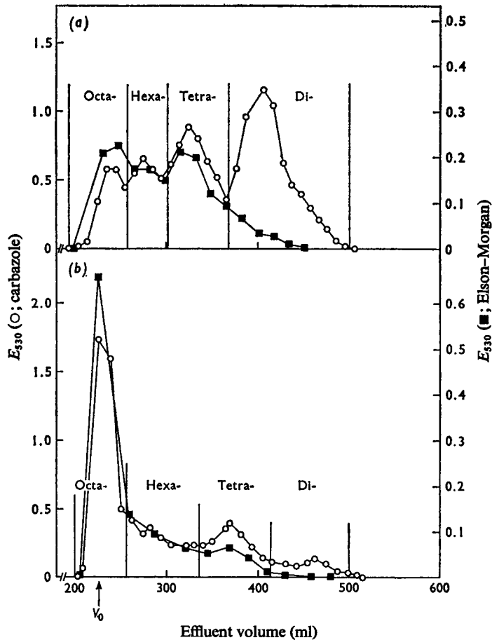
Fig. 6. Gel chromatography on Sephadex G-25 of products obtained on deamination of (a) heparin and (b) heparan sulphate. Effluent fractions were analysed for uronic acid (O) and hexosamine (■), and were then combined as indicated by the vertical lines. The pooled fractions are referred to in the text as indicated in the figures. The 'octasaccharide' fractions may contain larger components, emerging at the excluded volume ( V_0 ) of the column.
