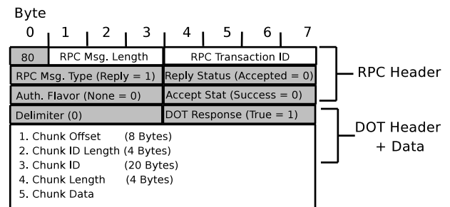
Figure 7: Ditto packet format. Shaded fields are invariant across Ditto responses and the Sniffer uses these to identify a Ditto chunk.
