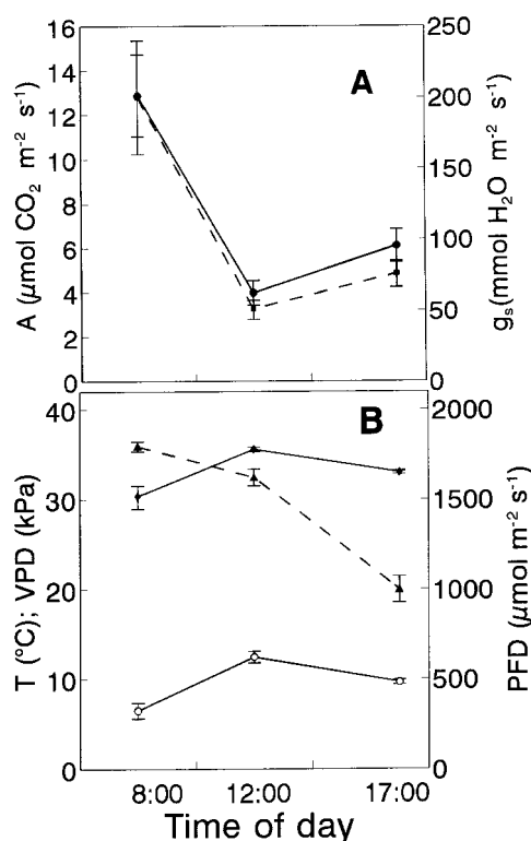
Figure 1. (A) Diurnal changes in net photosynthesis ( A ) (●) and stomatal conductance ( g_s ) (■) of sun leaves of Q. suber . (B) Diurnal variation in temperature (◆), solar radiation (PFD) (▲) and water vapor pressure deficit (○) during the experiment. Error bars represent the standard errors (SE) of at least five replicates.
