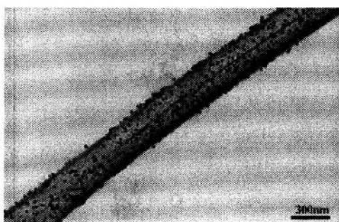
Figure 1.17 TEM image of a single \text{TiO}_2 nanotube coated with Au nanoparticles. (Reproduced from 96)
