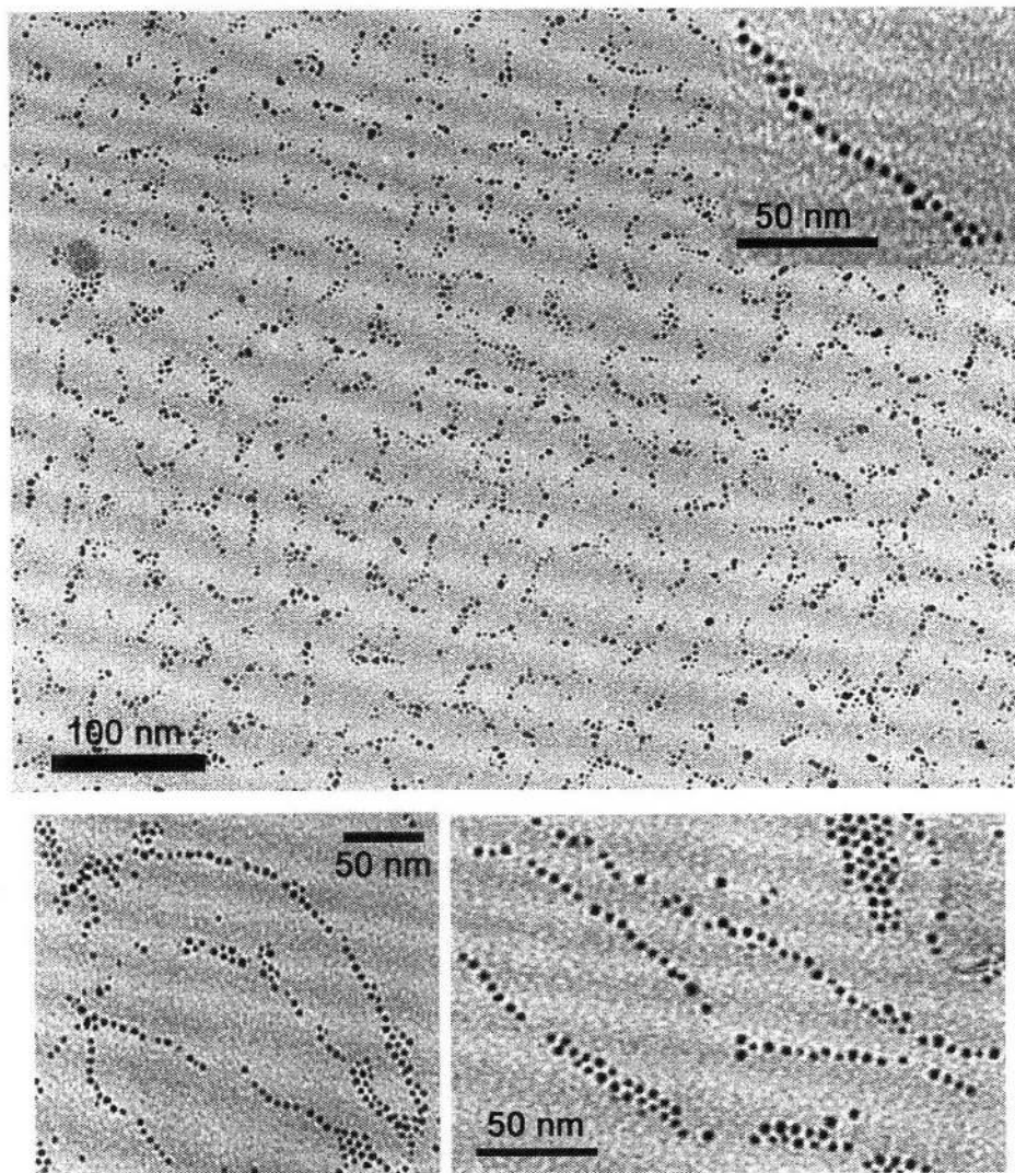
Figure 3.2 TEM images of chains obtained by pole functionalizing rippled NPs with MUA, then performing an interfacial polymerization with DAH. Precipitate at the interface was collected and dispersed for TEM imaging.
