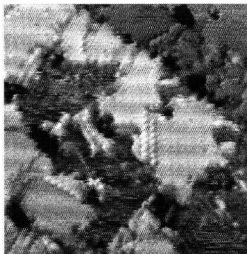
Figure 1.7 STM image of a phase-separated SAM consisting of n -decanethiol and an internally functionalized amide-containing thiol. The image is 300 Å x 300 Å in size. (Reproduced from 34)
