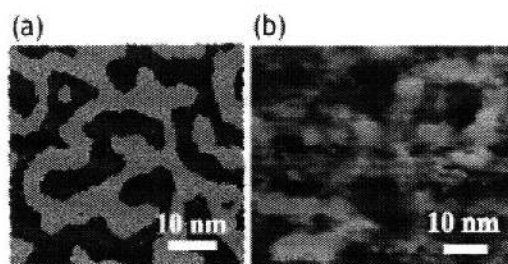
Figure 1.7 STM image of a phase-separated SAM consisting of n -decanethiol and an internally functionalized amide-containing thiol. The image is 300 Å x 300 Å in size. (Reproduced from 34)
