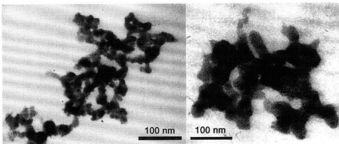
Figure 3.17 TEM images of large ball-like structures formed by performing a two-phase chaining reaction in which water-soluble NPs pole functionalized with MHDA and linked with sebacoyl chloride.
