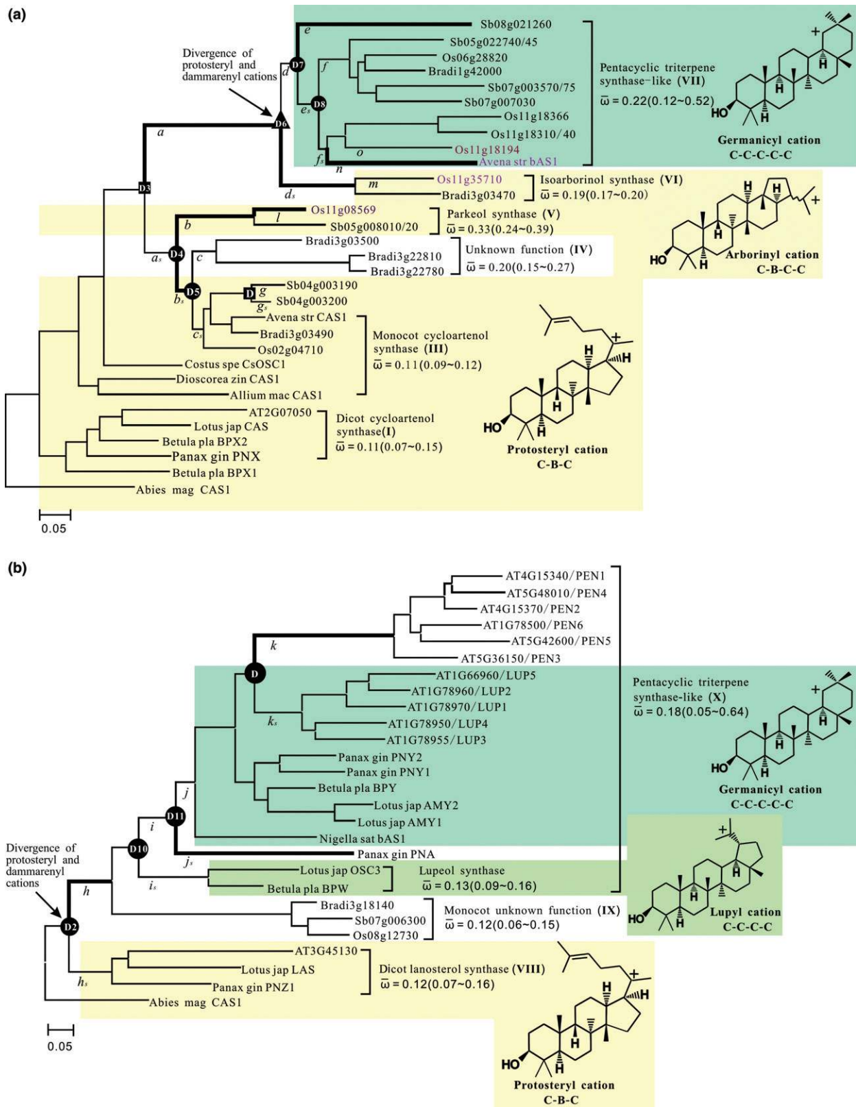
Fig. 7 Phylogenetic trees of cycloartenol synthase (CS)-derived (a) and lanosterol synthase (LS)-derived (b) oxidosqualene cyclases (OSCs). The 10 thick branches (a, b, b s , d s , e, h, i, j, k, l and n; see Table 3) indicate branches or genes evolving under positive selection with significant statistical support at P < 0.01 . Average estimates of the nonsynonymous : synonymous substitution ( dN/dS ) ratio, \bar{\omega} , are shown to the right of each function group. The conformation of products and the corresponding intermediate cations are shown on the right side of the figure. D1–D11 indicate the gene duplication events. Black squares indicate the tandem duplications, the triangle indicates the segmental or whole-genome duplication, and the dots indicate unknown types of duplications. [Correction added after online publication 25 January 2012: a new version of Fig. 7 is inserted here, to correct errors noted in the Early View version of this article.]
