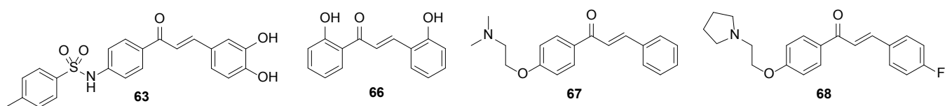
Figure 14: Structures of chalcones as AChE/BChE inhibitors.
