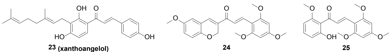
Figure 4: Structures of chalcones as Aurora kinase inhibitors.
