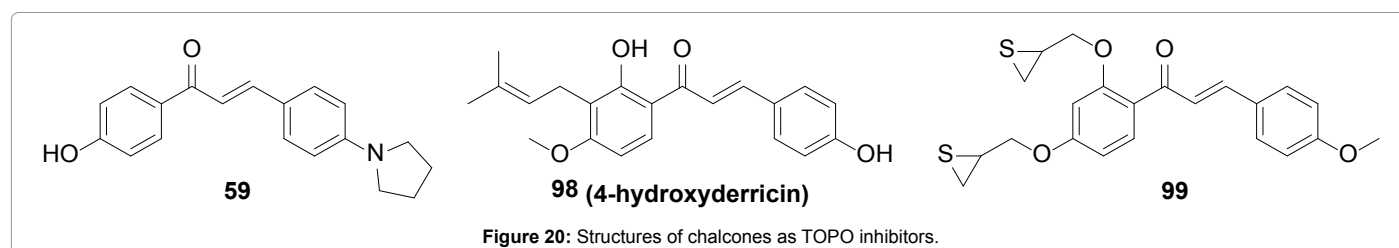
Figure 19: Structures of chalcones as inhibitors of ABC transporters.
