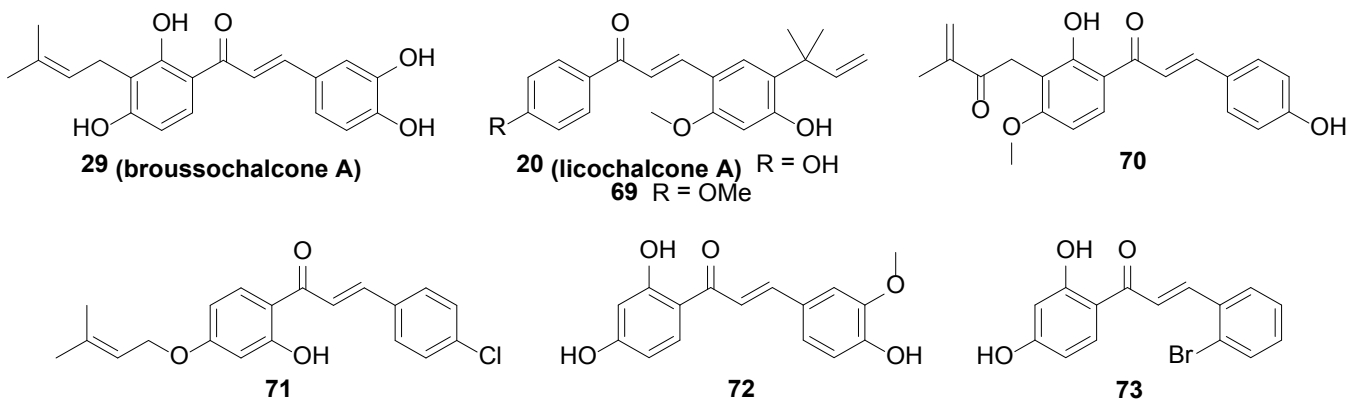
Figure 15: Structures of chalcones as PTP inhibitors.
