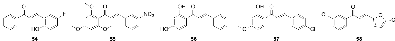
Figure 11: Structures of chalcones as TrxR and MAO inhibitors.
