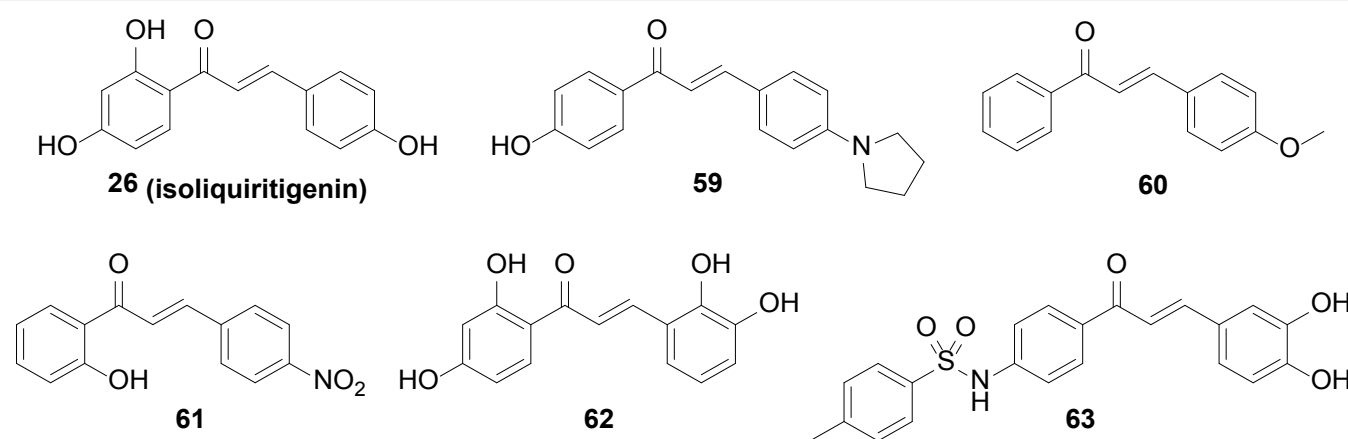
Figure 12: Structures of chalcones as inhibitors of proteases.
