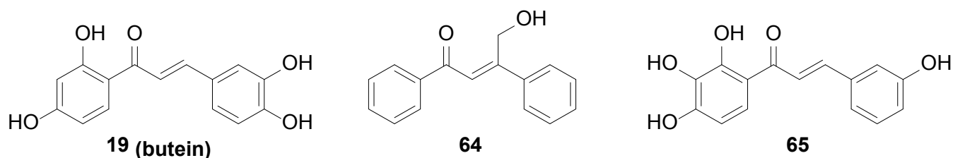
Figure 13: Structures of chalcones as HDAC inhibitors.
