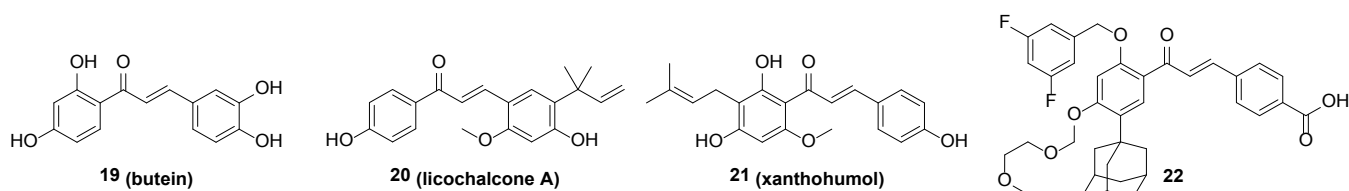
Figure 3: Structures of chalcones as IKK inhibitors.
