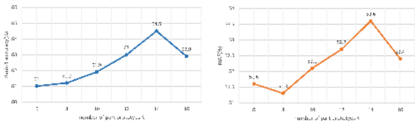
Figure 3. Comparison in Rank-1 accuracy and mAP with different settings of the part prototype number K on Occluded-Duke.
