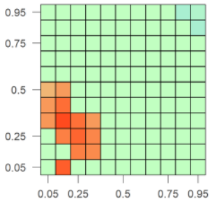
Fig. 3 Heat maps of CQ between daily S&P Green Bond and Financial Markets – COVID sub-sample.
