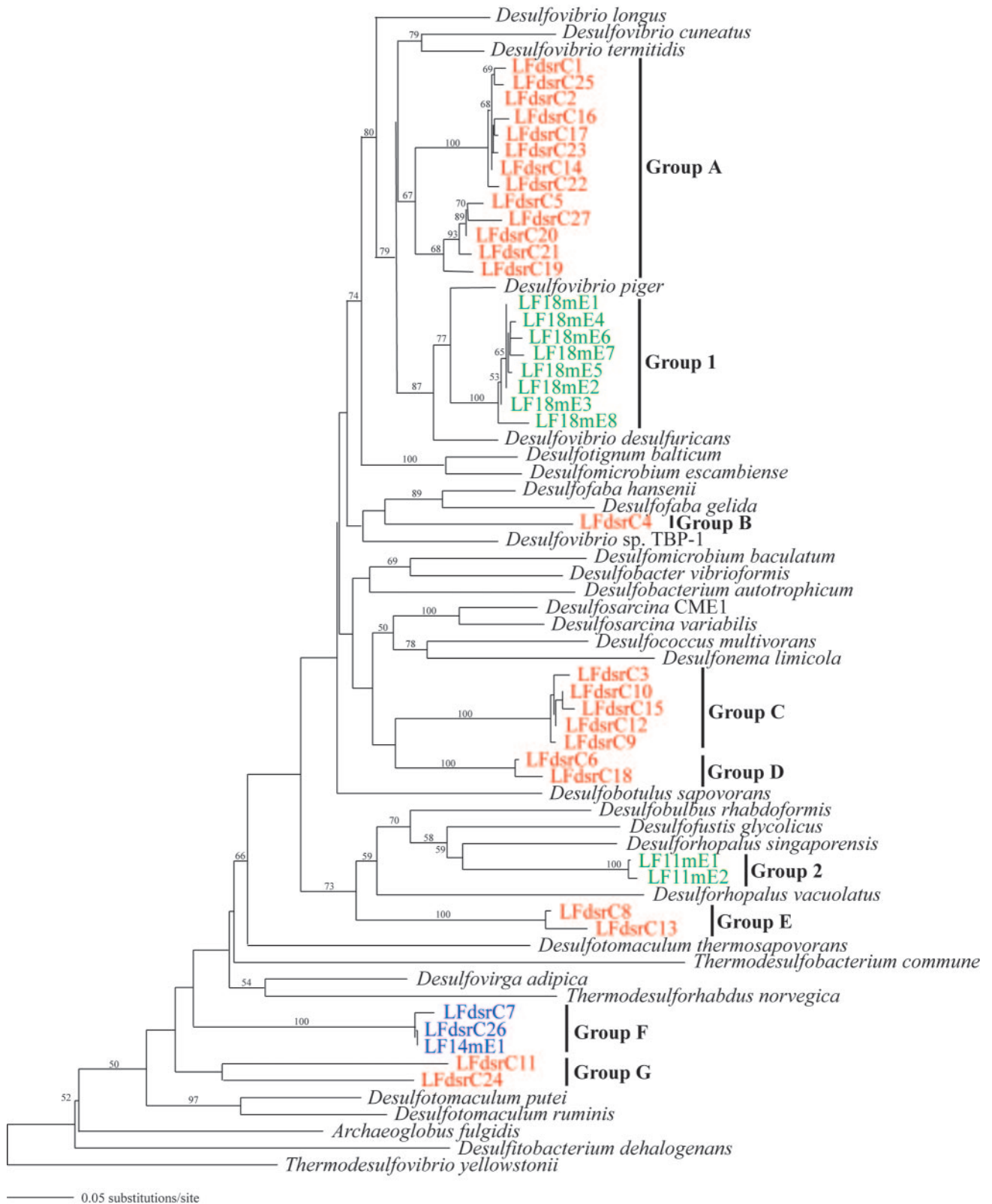
FIG. 2. Rooted neighbor-joining distance tree based on 215 nucleotide positions of the dsrA gene, using Thermodesulfovibrio yellowstonii as the outgroup. All designations beginning with LF are from Lake Fryxell. Environmental clone groups are represented in red, enrichment culture clones are represented in green, and the one group containing both enrichment and environmental clones is shown in blue. Bootstrap values of >50% are indicated.
