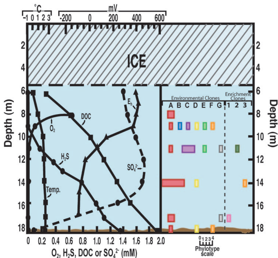
FIG. 3. Profile of Lake Fryxell, summarizing key physiochemical parameters (left) and the locations with depth of different groups of dsrA phylotypes in the water column (right). The widths of the colored boxes are proportional to the number of different phylotypes residing at a particular depth according to the scale bar on the bottom of the figure. Figure 2 shows the phylotypes in each group. The 14-m group 3 enrichment clone is identical in dsrA sequence to the group F environmental clone, LFdsrC26, found at 9 m and in the sediment. DOC concentrations are expressed as millimolar carbon (adapted from data in reference 29).
