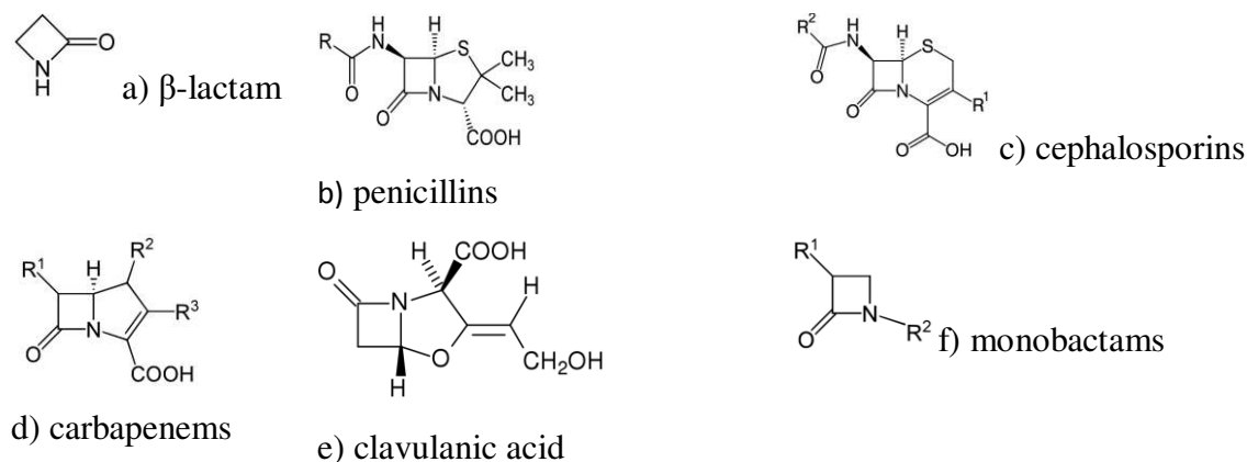
Figure 1. Chemical structures of the main groups of \beta -lactam family of antimicrobials; a- the \beta -lactam ring; b- general structure of penicillins; c- general structure of cephalosporins; d- general structure of carbapenems; e- example of \beta -lactamase inhibitor (clavulanic acid); f – core structure of monobactams
