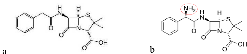
Figure 4. Structure of penicillin G (a) and example of aminopenicillin (ampicillin, b); in the circle indicated is the amino group (b)
