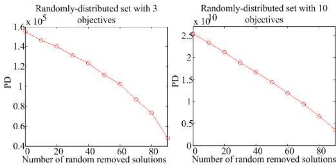
Fig. 8. Average PD values of randomly-distributed set with different numbers of solutions of dropped solutions for the 3- and 10-objective problems.
