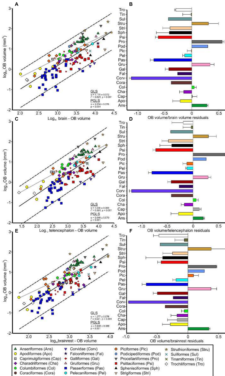
FIGURE 2 | Relative size of the OBs in birds. Scatterplots of the log-transformed volume of the OBs plotted as a function of either: (A) the log-transformed brain volume minus the volume of the OBs, (C) the log-transformed telencephalon volume minus the volume of the OBs or (E) ; the brainrest (brainstem, cerebellum, and thalamus) volume. The solid lines indicate the results from the generalized least-squares (GLS) regression, the
