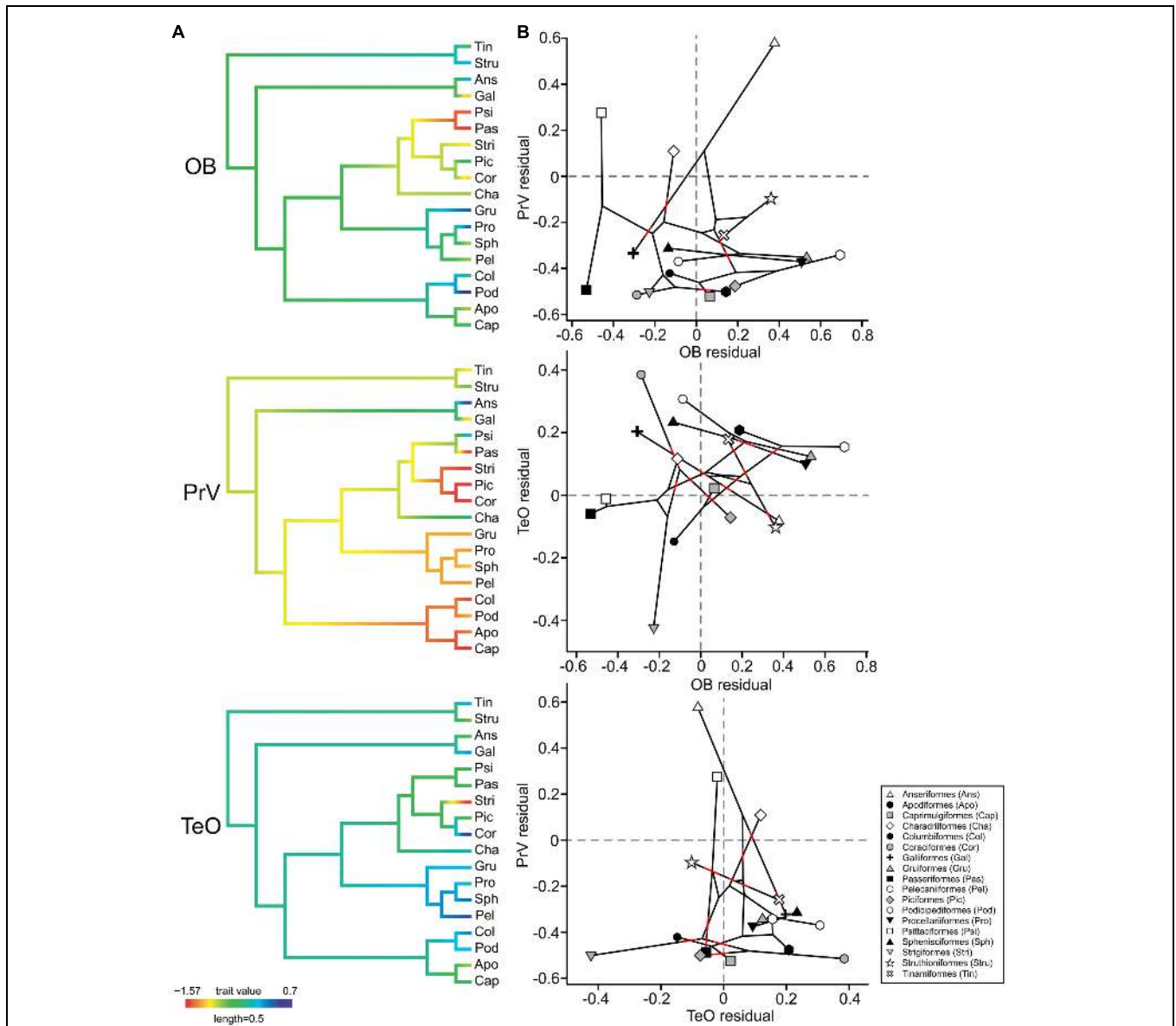
FIGURE 5 | Ancestral character estimates and residual plots for the OBs, the principal sensory nucleus of the trigeminal nerve (PrV), and the optic tectum (TeO). (A) Ancestral character estimates are plotted using the order averages for the relative size (expressed as the residuals of the best fitting PGLS model of each area against brain volume) of each sensory area (OB, PrV,
