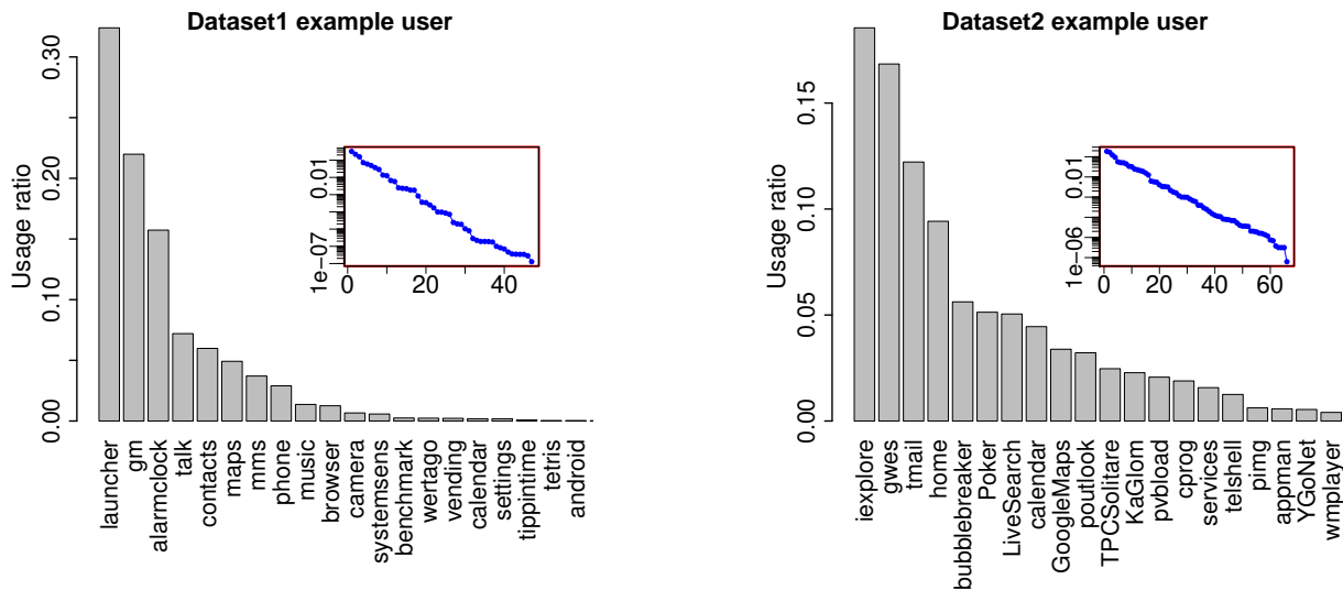
Figure 11: Relative time spent running each application for example users in each dataset. Inset is the semi-log plot of application popularity.
