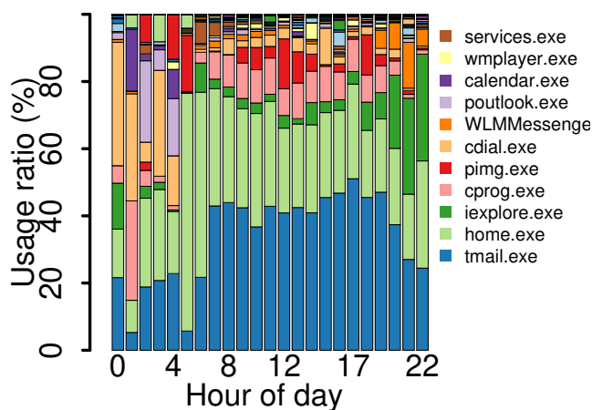
Figure 11: Relative time spent running each application for example users in each dataset. Inset is the semi-log plot of application popularity.
