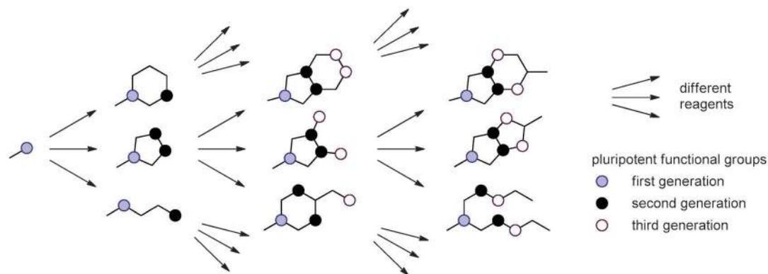
Scheme 2 The reagent based approach using pluripotent functional groups which are transformed into different products by different reagents in a branching pathway.
