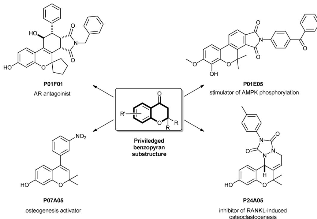
Scheme 5 Construction of diverse polycyclic skeletons embedded with the benzopyran motif by Park and colleagues displaying a wide variety of biological activity.
