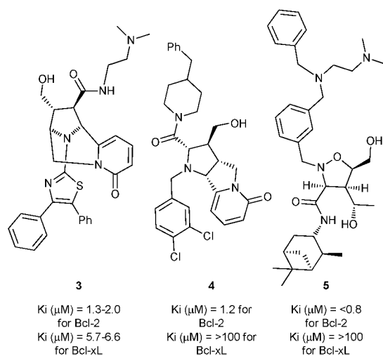
Fig. 5 Small molecule modulators of Bcl-2 family proteins. 61,62
