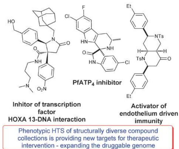
Fig. 1 Schematic illustrating some small molecule modulators of protein function discovered from screening structurally diverse libraries. 5-7
