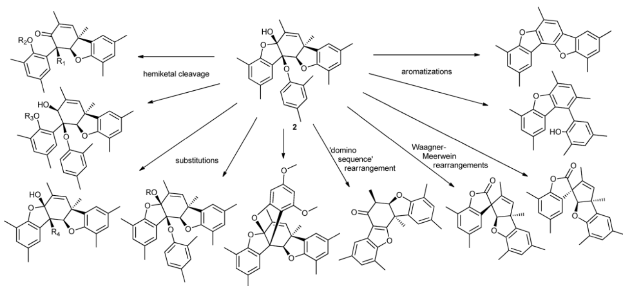
Scheme 1 Reagent based approaches using densely functionalized molecules. (a) Tan and co-workers used a various set of pairing reactions to create a library of 190 compounds based on 10 distinct scaffolds. 20 (b) Waldvogel and co-workers used a set of reagent-induced rearrangements and transformations to create 13 compounds based on 9 complex polycyclic skeletons. 38
