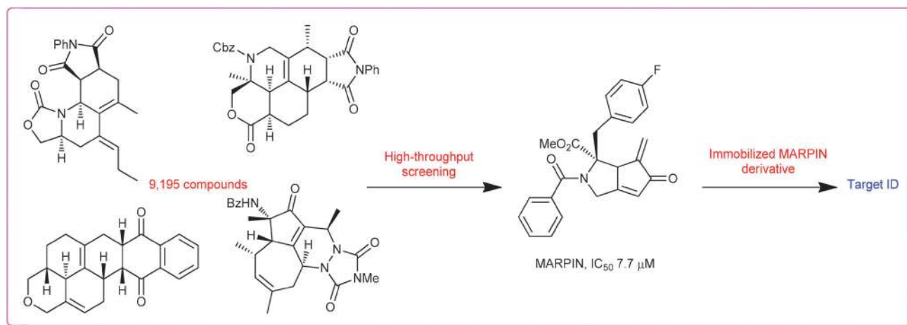
Scheme 4 Screening of DOS library identified a novel DNA checkpoint inhibitor, MARPIN. 66
