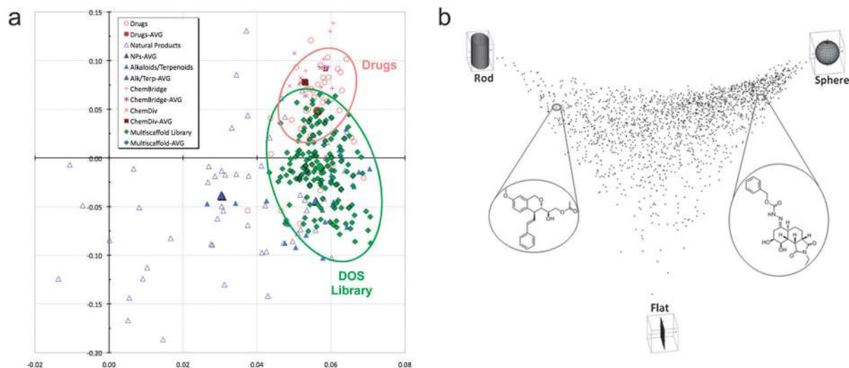
Fig. 2 Diversity assessment of compound collections. (a) Principal component analysis (PCA) of the 40 top-selling drugs (red circles), 60 diverse natural products (open blue triangles), 20 polycyclic alkaloids and terpenoids (filled blue triangles), 20 ChemBridge and ChemDiv library members (crosses), and 190 members of a DOS library synthesized by Tan and coworkers (green diamonds). 20 The DOS library spans a large area of chemical space distinct from the area populated by approved drugs and commercial compound collections. Adapted with permission from ref. 20. (b) Principle moments of inertia (PMI) analysis of the 2070 membered diversity compound collection of the Center for Chemical Methodology and Library Development at Boston University (CMLD-BU). 21 The analysis reveals a significant predominance of spherically shaped compounds over flat compounds typically found in commercial collections. Adapted with permission from ref. 21.
