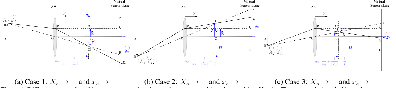
(a) Case 1: X_s \rightarrow + and x_s \rightarrow - (b) Case 2: X_s \rightarrow - and x_s \rightarrow + (c) Case 3: X_s \rightarrow - and x_s \rightarrow - Figure 4. Different cases of world-to-sensor mapping for a subaperture positioned at positive X axis. The same relations hold good even for subapertures positioned at negative X axis due to symmetry about optical axis. (Variables having negative values are marked with (-) )
