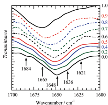
Figure 3. ATR-IR spectra in the amide I region of 7 g L -1 lysozyme solutions in D 2 O/ d 6 -DMSO solutions containing 0.0 \leq \varphi_{\text{DMSO}} \leq 1.0 as indicated. The arrows indicate the positions of some characteristic bands: 1684 cm -1 (turns), 1665 cm -1 (free carbonyl groups, i.e. not H-bonded to other amino acids), 1648 cm -1 ( \alpha -helix), 1636 cm -1 (intramolecular \beta -sheet), 1622 cm -1 (intermolecular \beta -sheet). For presentation purposes the spectra have been shifted in the vertical direction.
